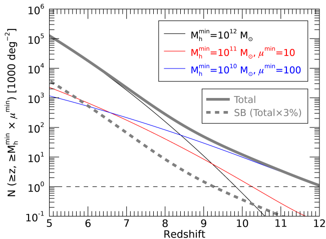
Figure 6. Cumulative surface densities of DM halos per 1000 \text{deg}^2 as predicted by the the standard \Lambda CDM model. The black line indicates the cumulative surface density of \geq 10^{12} M_{\odot} halos down to given redshifts while the blue and red lines plot the corresponding numbers for \geq 10^{11} M_{\odot} halos gravitationally lensed by a factor of \geq 10\times ( \mu \geq 10 ) and for \geq 10^{10} M_{\odot} halos lensed by a factor of \geq 100\times ( \mu \geq 100 ), respectively. According to the calculation by Zackrisson et al. (2015), when the source redshift is above \sim 5 , the corresponding lensing probability is roughly constant and \sim 10^{-4} for \mu \geq 10 and \sim 10^{-6} for \mu \geq 100 along an average line of sight. These probabilities have been multiplied with the \geq 10^{11} and \geq 10^{10} M_{\odot} halo surface densities. The thick grey line plots the total surface density of the three halo populations combined while the thick grey dashed line plots 3% of the total number, comparable to the starburst fraction estimated at lower redshift (e.g., Béthermin et al. 2017). The halo comoving number density was computed with the Press-Schechter formalism (Press & Schechter 1974). The horizontal dashed line corresponds to N = 1 .
