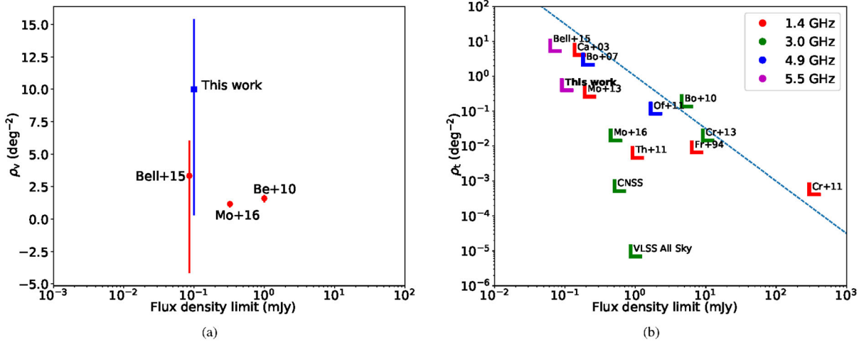
Figure 8. Left-hand panel: the density of significantly variable radio sources as a function of flux density in surveys made at \sim 5 and 3 GHz by Bell et al. (2015), this work, Becker et al. (2010) and Mooley et al. (2016). The density of significantly variable sources is consistent within a 1\sigma Poisson error for surveys done in the past. Right-hand panel: the density of transient radio sources in surveys conducted at 1.4 GHz (Frail et al. 1994; Carilli, Ivison & Frail 2003; Croft et al. 2011; Thyagarajan et al. 2011; Mooley et al. 2013), 3 GHz (Bower et al. 2010; Croft, Bower & Whysong 2013; Mooley et al. 2016, CNSS pilot, CNSS, VLSS), 4.9 GHz (Bower et al. 2007; Ofek et al. 2011), and 5.5 GHz (this work, Bell et al. 2015) as a function of flux density. The dashed blue line shows \rho_t \propto S^{-3/2} . This is the relation for a Euclidean population.
