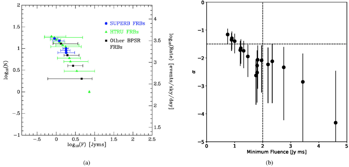
Figure 6. Left-hand panel: the source count distribution of Parkes FRBs. The sky rate is indicated on the right, normalized to rate of 1.7 \times 10^3 FRBs sky ^{-1} d ^{-1} for \mathcal{F} > 2 Jy ms (see Section 5.4). Right-hand panel: the slope \alpha of the integral source counts obtained using the maximum-likelihood method (Crawford et al. 1970). We obtain a slope of \alpha = -2.2^{+0.6}_{-1.2} for FRBs above a fluence completeness limit of 2 Jy ms in our updated sample of 19 FRBs. The vertical dashed line indicates the fluence completeness limit and the horizontal dashed line indicates \alpha = -3/2 , the slope expected for constant space density sources distributed in a Euclidean Universe.
