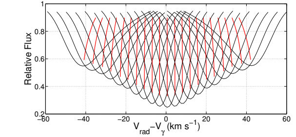
Figure 4. Example of LSD profiles and bisectors computed from model spectra of RR Lyrae (that corresponds to \phi=0.213 , or spectrum number 087 in Fossati et al. 2014) with pulsation velocities from -50 to +50 \text{ km s}^{-1} with a step 5 \text{ km s}^{-1} .
