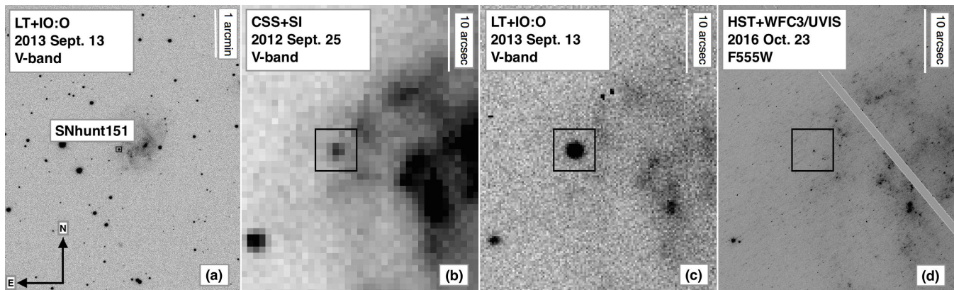
Figure 1. V- and F555W-band images of SNhunt151 in UGC 3165 obtained with the Liverpool Telescope+IO:O on 2013 September 13 (a,c), the Cassegrain reflector+SI on 2012 September 25 (b), and HST+WFC3/UVIS on 2016 October 23 (d). The location of the transient is indicated.
