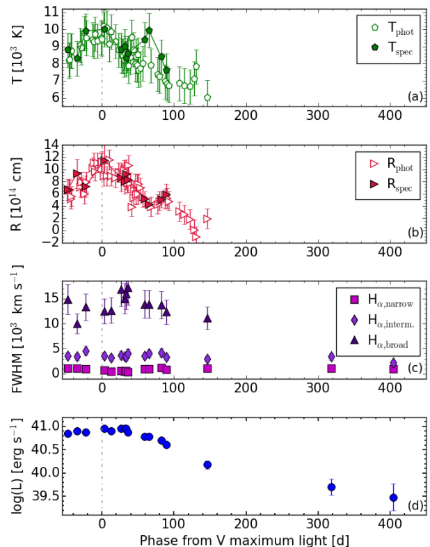
Figure 8. (a): Evolution of the best-fit blackbody temperatures. (b): Evolution of the radius of the photosphere. The solid line connects the temperature and radius measurements. (c): FWHM evolution for the broad and narrow H \alpha emission. (d): Evolution of the total luminosity of H \alpha . The dot-dashed vertical line indicates the V-band maximum light of SNhunt151. A conservative uncertainty of about \pm 1000 K for the temperature has been assumed.
