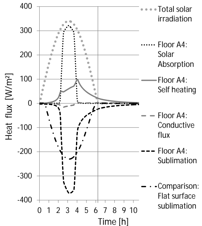
Fig. 5. Heat flux patterns for fracture A4 at a heliocentric distance of 2.0 AU and a plane angle \eta=30 deg for one diurnal period of 12.4 h. The vertical lines at 0h and 6.2h indicate local morning and evening terminator. The coarse dotted grey line denotes the incident total solar irradiation, while the smaller black dotted line outlines the absorbed heat flux by the fracture floor. The grey continuous line shows the self-heating by infrared radiation, emitted from the fracture side walls, which impinges on the fracture floor: a positive value indicates a net heat flux direction towards the fracture floor. The grey dashed line illustrates the heat exchange with underlying nucleus layers through conductive and radiative transport. The black dashed line marks the local heat sink by sublimation phase change processes. For comparison, the dash-dotted line marks the sublimation pattern of a flat surface with identical thermophysical properties. The sublimation front is located directly at the surface of the fracture floor. Remarks: (1) The heat fluxes are related to 1 \text{ m}^2 sublimating fracture floor. Owing to the concave structure of geometry A4 and the decreasing width with depth, the fracture top sums up to 4 \text{ m}^2 . (2) The fractured terrain absorbs about 4 % more thermal energy than a flat surface because scattered irradiation is absorbed.
