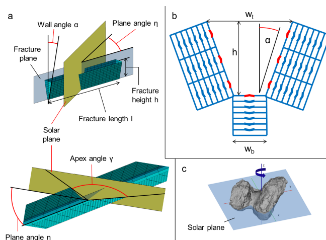
Fig. 3. Parametric model definition for a generic fracture: a) plane definitions, b) schematic nodal breakdown of a parametrised fracture with radiative heat exchange (red arrows) and effective conductive thermal fluxes (blue arrows), and c) solar plane with respect to the rotational axis of 67P at equinox.
