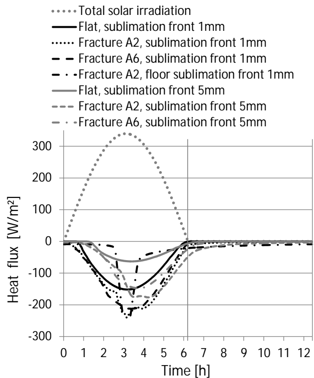
Fig. 10. Diurnal irradiation and sublimation fluxes for fully subliming fractures A2 and A6. The grey dotted line shows the solar irradiation for one diurnal revolution at 2 AU as a positive heat source, the sublimation heat sinks are depicted for two sublimation fronts of 1mm and 5mm depth. The vertical line at 6.2h denotes the terminator.
