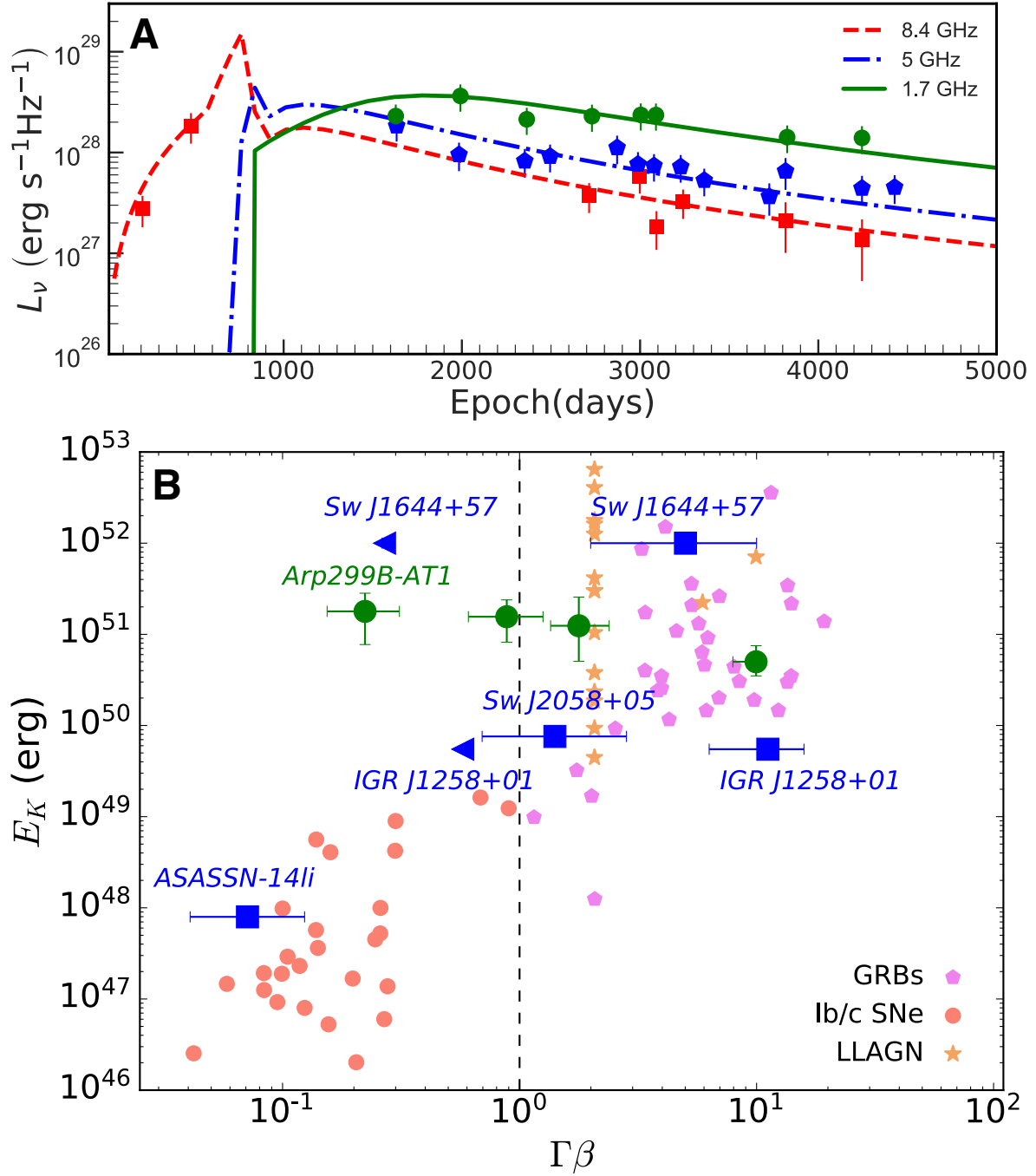
Figure 2. Radio properties of Arp 299-B AT1. (A) Radio luminosity evolution of Arp 299-B AT1 at 1.7 (circles), 5.0 (pentagons) and 8.4 GHz (squares) spanning more than 12.1 years of observations, along with modeled radio light curves, using hydrodynamic and radiative simulations for a tidal disruption event (TDE) launched jet (16). The day zero corresponds to 2004 Dec. 21.6. (B) Intrinsic (beaming-corrected) jet kinetic energy, E_K , versus outflow speed ( \Gamma\beta , where \Gamma = (1-\beta^2)^{-1/2} is the bulk Lorentz factor of the outflow and \beta = v/c ), from radio observations of gamma-ray bursts (GRB), supernovae (SNe), low-luminosity active galactic nuclei (LLAGN), and TDEs (4, 16, 19-21, 32). The large circles show, from right to left, the inferred loci for Arp 299-B AT1 at four different epochs in the observer’s frame: just after the jet is launched by the TDE, and \sim 1 , \sim 12 , and \sim 760 days thereafter. For the LLAGN sample, we have assumed a constant jet kinetic power over 10 yr. The triangles indicate upper limits for the expansion speed of IGR J1258+01 (20) and Sw J1644+57 (21).
