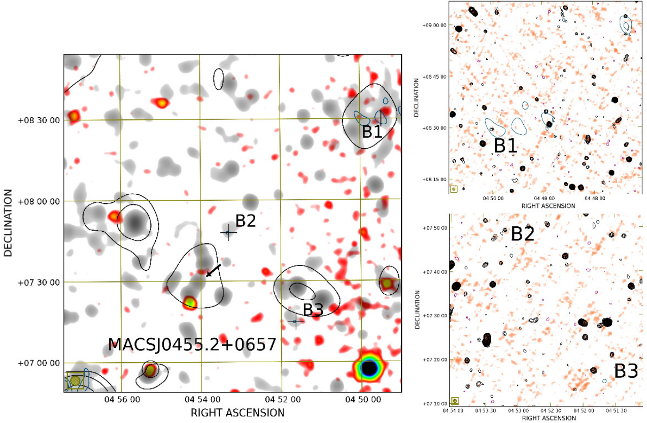
Figure 8. Region B. Left panel: SRT contours ( -60 mJy/beam, 60 mJy/beam, 150 mJy/beam, 500 mJy/beam, negative in magenta and positive in black; resolution 13.9' \times 12.4' ) and SRT+NVSS after compact sources subtraction contours (in blue, starting from 3\sigma and the remaining increasing by a factor \sqrt{2} ; \sigma=2.5 mJy/beam, resolution 3.5' \times 3.5' ) overlaid on X-ray emission from the RASS in red colours and radio emission from the SRT+NVSS (resolution 3.5' ) in gray colours. Right panels: NVSS contours -3\sigma (magenta, \sigma=0.45 mJy/beam), 3\sigma , and increasing by a factor \sqrt{2} (black) overlaid on the TGSS in colours. The black arrow marks the region shown in the zoom of Fig. 9. The colorbars are the same as in Fig. 7.
