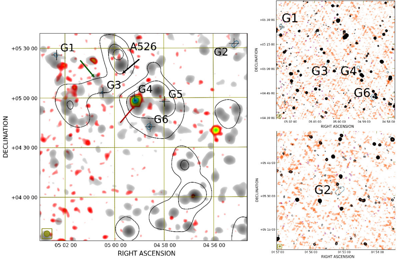
Figure 14. Region G. Left panel: SRT contours ( -60 mJy/beam, 60 mJy/beam, 150 mJy/beam, 500 mJy/beam, negative in magenta and the remaining increasing by a factor \sqrt{2} ; \sigma=2.5 mJy/beam, resolution 3.5' \times 3.5' ) overlaid on X-ray emission from the RASS in red colours and radio emission from the SRT+NVSS (resolution 3.5' ) in gray colours. Right panels: NVSS contours -3\sigma (magenta, \sigma=0.45 mJy/beam), 3\sigma , and increasing by a factor \sqrt{2} (black) overlaid on the TGSS in colours. The black and red arrow mark respectively the locations of the galaxy cluster ZwCl0457.0+0511 and of the compact source PMN J0459+0455, while the green arrow a bridge of radio emission detected by SRT. The colorbars are the same as in Fig. 7.
