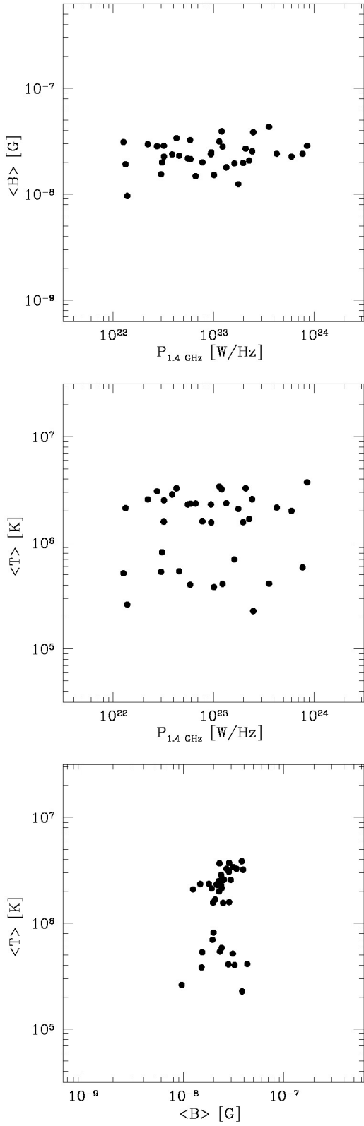
Figure 23. Top panel: mean volume-weighted magnetic field \langle B \rangle versus P_{1.4\text{GHz}} . Middle panel: mean temperature \langle T \rangle versus P_{1.4\text{GHz}} . Bottom panel: \langle T \rangle versus \langle B \rangle .
