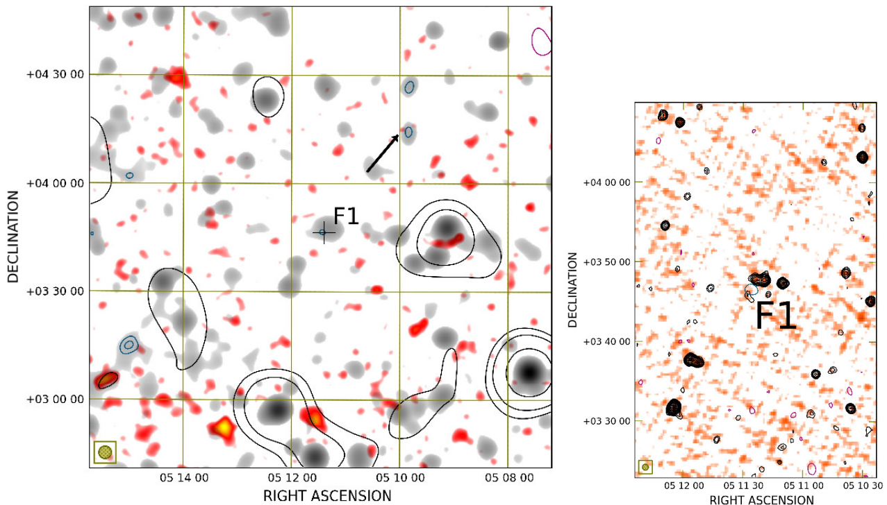
Figure 13. Region F. Left panel: SRT contours (-60 mJy/beam, 60 mJy/beam, 150 mJy/beam, 500 mJy/beam, negative in magenta and positive in black; resolution 13.9' \times 12.4' ) and SRT+NVSS after compact sources subtraction contours (in blue, starting from 3\sigma and the remaining increasing by a factor \sqrt{2} ; \sigma=2.5 mJy/beam, resolution 3.5' \times 3.5' ) overlaid on X-ray emission from the RASS in red colours and radio emission from the SRT+NVSS (resolution 3.5' ) in gray colours. Right panel: NVSS contours -3\sigma (magenta, \sigma=0.45 mJy/beam), 3\sigma , and increasing by a factor \sqrt{2} (black) overlaid on the TGSS in colours. The black arrow marks the position of the candidate giant radio galaxy we found (see § B). The colorbars are the same as in Fig. 7.
