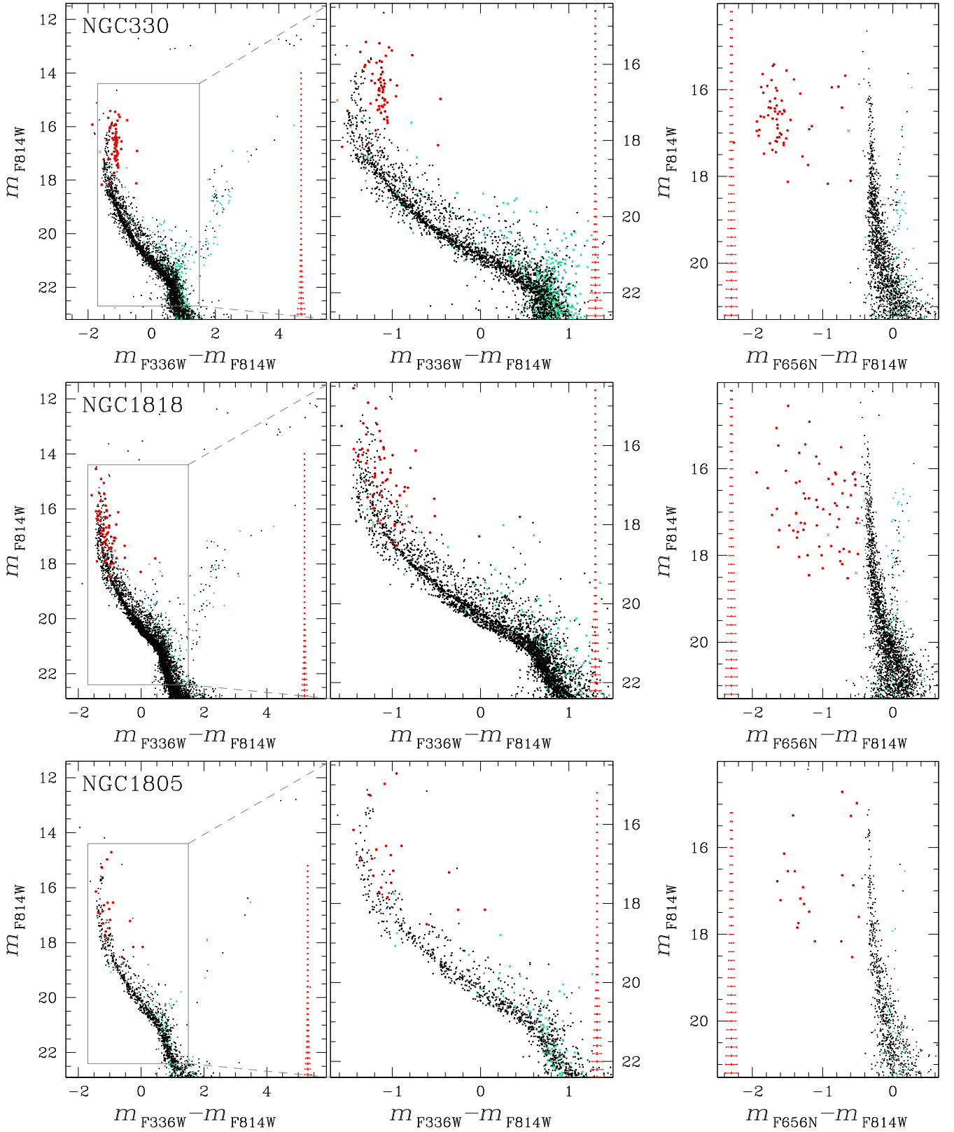
Figure 2. Collection of CMDs for stars in the field of view of NGC 330, NGC 1818, and NGC 1805. The left-hand panels show the m_{F814W} versus m_{F336W} - m_{F814W} CMD for stars in the cluster field (black points) and in the reference field (aqua crosses). The middle panels are a zoom-in of the left-hand-panel CMDs around the upper MS and the MSTO. The right-hand panels plot m_{F814W} against m_{F656N} - m_{F814W} for stars in the cluster field (black points) and in the reference field (aqua crosses). Candidate H\alpha emitters in the cluster field and in the reference field have been selected in the right-hand-panel CMDs and are represented with red circles and brown crosses, respectively, in all the diagrams of this figure. The clusters are sorted in order of increasing age.
