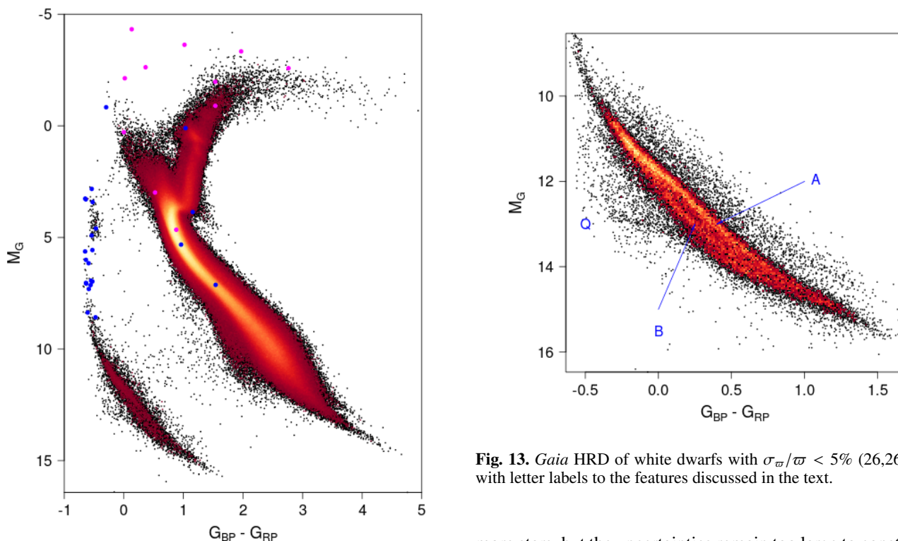
Fig. 12. North Galactic Pole HRD ( b > 50^\circ , 2,077,925 stars) with literature central planetary nebula stars (blue) and post-AGB stars (magenta).
