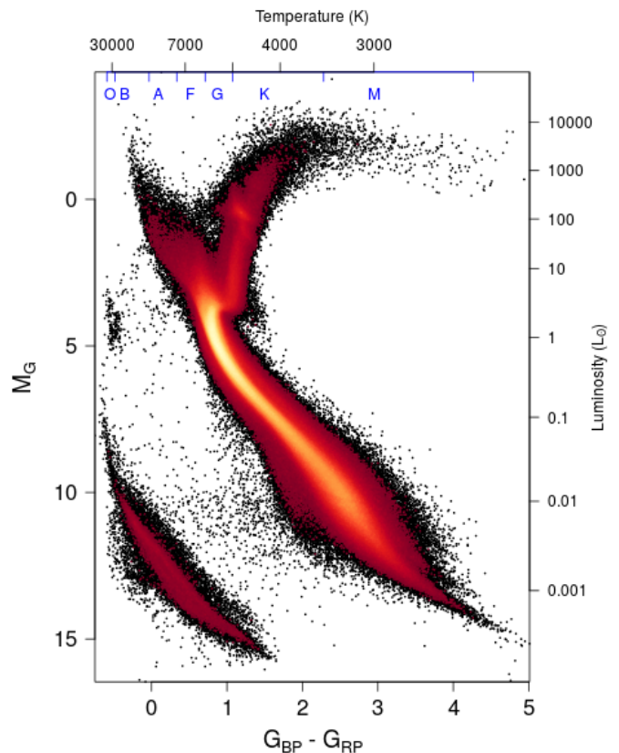
Fig. 5. Gaia HRD of sources with low extinction ( E(B - V) < 0.015 mag) satisfying the filters described in Sect. 2.1 (4,276,690 stars). The colour scale represents the square root of the density of stars. Approximate temperature and luminosity equivalents for main-sequence stars are provided at the top and right axis, respectively, to guide the eye.
