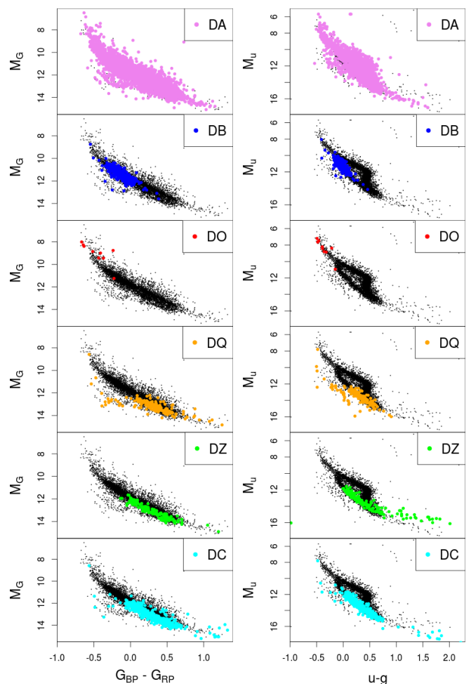
Fig. 16. SDSS white dwarfs per spectral type (DA: hydrogen; DB: neutral helium; DO: ionised helium; DQ: carbon; DZ: metal rich; and DC: no strong lines). panel a): Gaia photometry, panel b): SDSS photometry.
