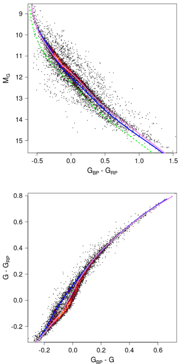
Fig. 14. Gaia HRD of white dwarfs with \sigma_{\pi}/\pi < 5\% and \sigma_{G_{BP}} < 0.01 and \sigma_{G_{RP}} < 0.01 (5,781 stars) overlaid with white dwarf evolutionary models. Magenta : 0.6 M_{\odot} pure H; green dashed : 0.8 M_{\odot} pure H; and blue : 0.6 M_{\odot} pure He. a): HRD. b): Colour-colour diagram.
