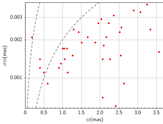
Fig. A.10. Standard uncertainties on the mean cluster parallax determinations. The curves represent the 100 and 500 \sigma significance levels when only the standard uncertainties are considered.
