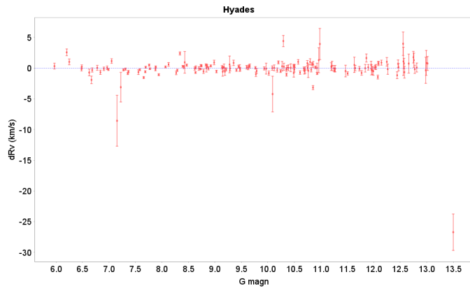
Fig. A.5. Differences between the predicted and observed radial velocities in the Hyades cluster as a function of G magnitude.
