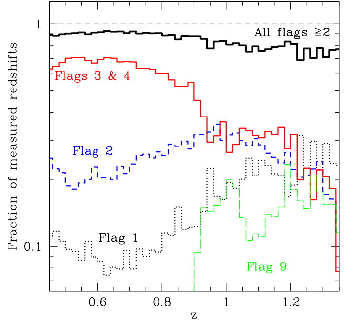
Fig. 9. Quality of the VIPERS redshift measurements for different redshifts. Specifically, the plot shows how the fraction of measurements for different quality flags changes as a function of redshift. Note how the “reliable sample”, i.e. that with quality flag \geq 2 , to be used for statistical analyses, shows a stable measured fraction out to the limit of the survey.
