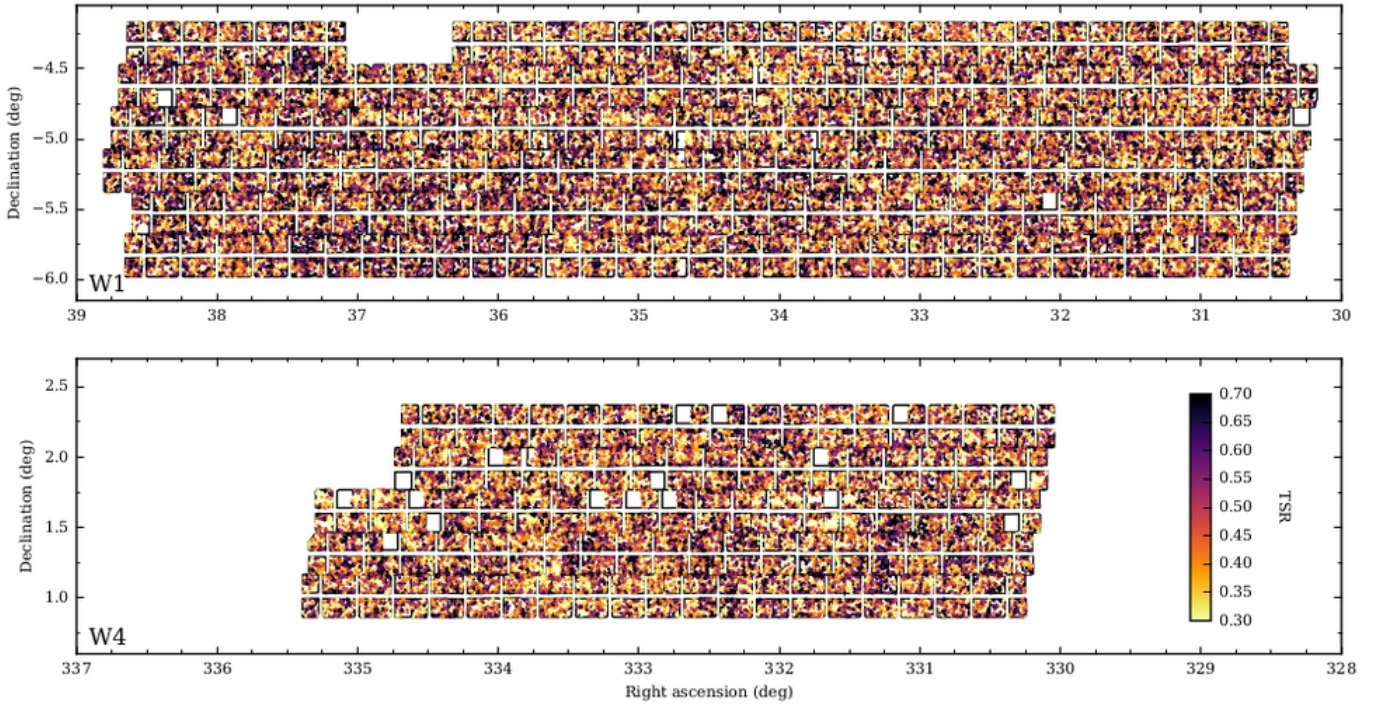
Fig. 5. Angular distribution over the survey areas of the target sampling rate (TSR, colour scale), estimated locally for each galaxy as described in the text. In this plot, each value has been smoothed on a scale of 2 arcmin to enhance the (inverse) relationship of the TSR with the projected large-scale structure in the galaxy distribution.
