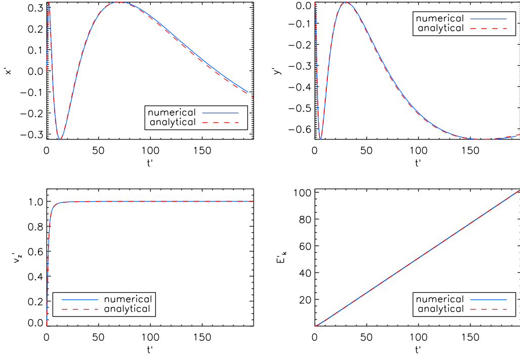
Figure 3. Particle position (top panels), velocity (bottom-left panel), and energy density (bottom-right panel) as a function of time for a charged particle in generic electric and magnetic fields. Quantities are plotted in the frame where both electric and magnetic fields are along the z axis.
