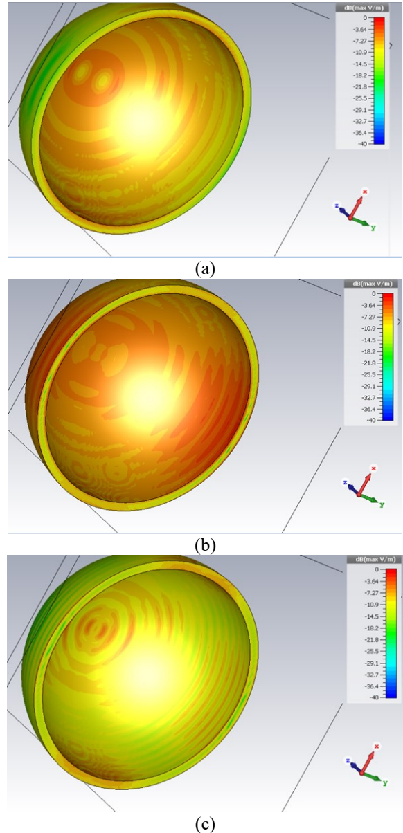
Figure 3. E-field transparency through Plexiglas vacuum window at (a) 4 GHz, (b) 6 GHz, and (c) 8 GHz. The red-coloured parts have a greater transparency (see color-coded vertical scale in the insets).
