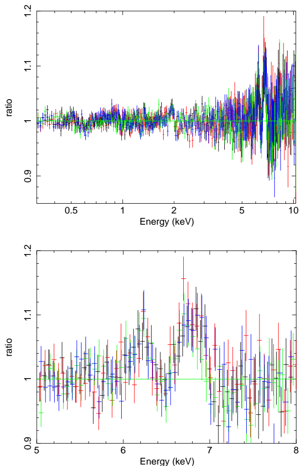
Fig. 3. Data/model ratio of the fit over the 0.3–10 keV energy range of the four 2014 XMM-Newton /pn spectra with the baseline relativistic reflection model (model \mathcal{A} ). The best fit parameters are reported in Table 3. Black: March 18, red: March 20, green: March 22, and blue: March 24. Top panel: the full 0.3–10 keV energy range. Bottom panel: zoom on the Fe K\alpha complex.
