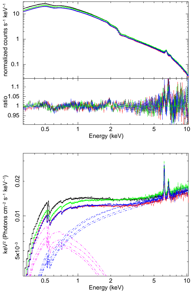
Fig. 4. Fit over the 0.3–10 keV energy range of the four 2014 XMM-Newton /pn spectra with the baseline Comptonization model (model \mathcal{B} ). The fit parameters are reported in Table 4. Black: March 18, red: March 20, green: March 22, and blue: March 24. Top panel: data and data/model ratio. Bottom panel: unfolded spectra where the contributions of the model components are displayed. The following color code for the emission components (dot-dashed curves) is used: magenta for the soft Comptonization (COMPTT), blue for the CUT-OFF POWER-LAW (hot Comptonization). For clarity purposes, we have not displayed the Fe K line components.
