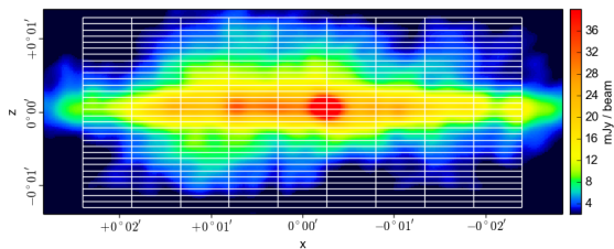
Fig. 13. Image of NGC 891 with indication of the boxes used for computing the average intensities, at different distances from the major axis of the galaxy’s projected disk, and in 9 different strips along the major axis.
