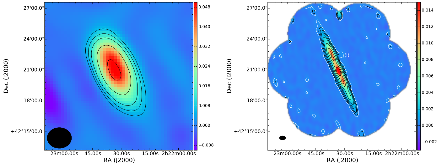
Fig. 5. AMI maps of NGC 891 observed at a central frequency of 15.5 GHz with the Small Array (SA) at 142'' \times 121'' resolution (left) and the Large Array (LA) at 36'' \times 24'' resolution (right). For the SA image, contours are at 3, 5, 8, 16, 32, 64 \times \sigma where \sigma = 1.5 \text{ mJy/beam} is the rms noise level. For the LA image, contours are at 3 (white), 5, 8, 12, 18, 36, 72, 108 \times \sigma where \sigma = 0.11 \text{ mJy/beam} is the rms noise level. The colour scales are in units of Jy/beam. The sizes of the synthesized beams are shown by the filled ellipses in the bottom left corners.
