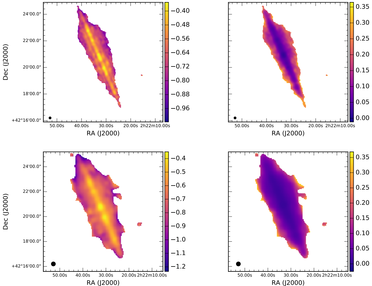
Fig. 10. Spectral index (left) and error map (right) of NGC 891 between 146 MHz and 1.5 GHz at resolutions of 10'' (top) and 20'' (bottom).
