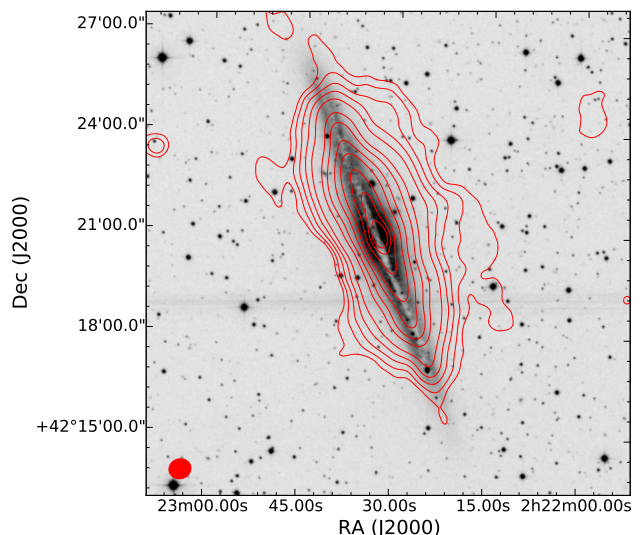
Fig. 4. LOFAR map of NGC 891 at a resolution of 40.0'' \times 35.7'' shown by the filled ellipse in the bottom left, overlaid onto an optical image from the Digitized Sky Survey. Contours are at 3, 5, 8, 12, 18, 32, 44, 88, 164, 200 \times \sigma where \sigma = 1.1 mJy/beam is the rms noise level.
