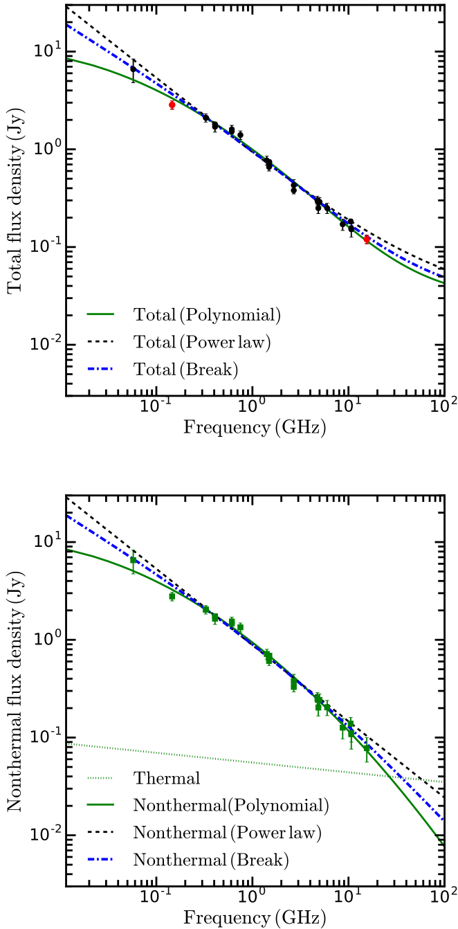
Fig. 9. Top: Integrated total flux densities of NGC 891 as listed in Table 5. The two new total flux densities from this paper are marked in red. Bottom: Integrated nonthermal flux densities of NGC 891 after subtracting an estimate of the optically thin thermal free–free emission (shown as the green dotted line) from the total flux densities. The black dashed, solid green, and blue dashed–dotted lines in the bottom panel show the best-fit power law, second-order polynomial model, and spectral break model to the nonthermal emission, respectively. The corresponding lines in the top panel show the expected total flux density after adding the thermal free–free emission to the different models of the nonthermal spectrum.
