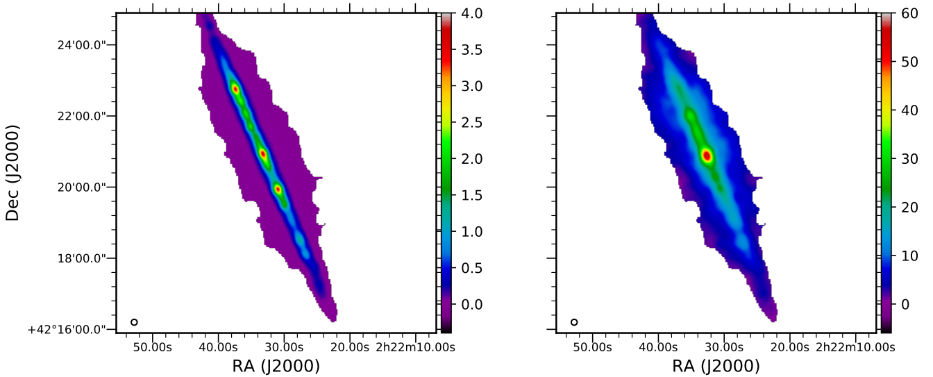
Fig. 7. Thermal map (left) and nonthermal map (right) of NGC 891 at 146 MHz at a resolution of 12'' , shown by the circle in the bottom left corner. The colour scale is in mJy/beam.
