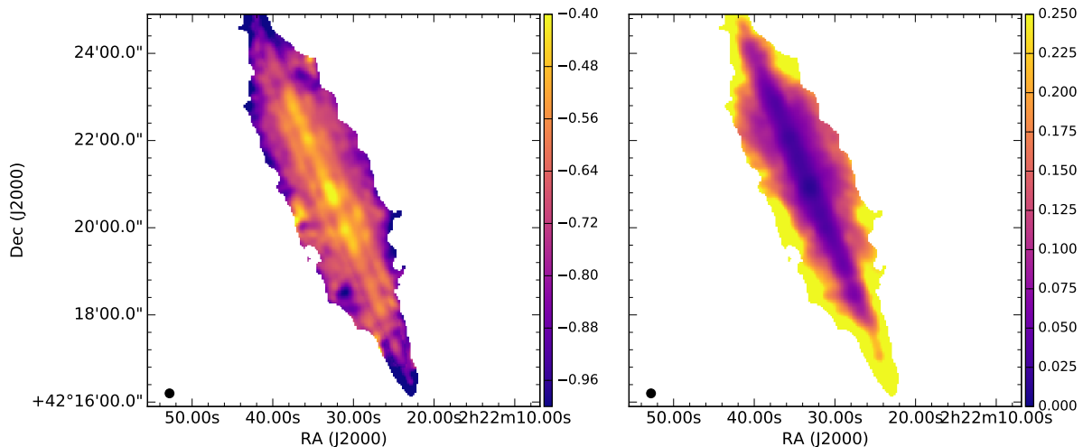
Fig. 11. Maps of nonthermal spectral index (left) and corresponding error map (right) between 146 MHz and 1.5 GHz at 12'' resolution. The beam is shown in the bottom left corner.
