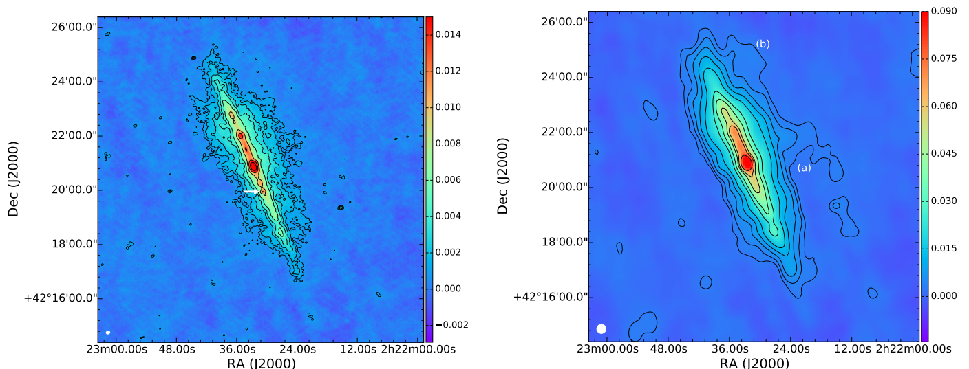
Fig. 3. LOFAR maps of NGC 891 observed at a central frequency of 146.4 MHz with a bandwidth of 34.4 MHz at two different resolutions. Left: Resolution of 8.3'' \times 6.5'' (shown by the filled ellipse in the bottom left corner). Contours are at 3, 5, 8, 12, 18, 32, 44, 64 \times \sigma where \sigma = 0.29 mJy/beam is the rms noise level. The location of SN1986J is shown by the white arrow. Right: Resolution of 20'' \times 20'' (shown by the filled ellipse in the bottom left corner). Contours are at 3, 5, 8, 12, 18, 32, 44, 64, 76 \times \sigma where \sigma = 0.8 mJy/beam is the rms noise level. The features denoted by ‘(a)’ and ‘(b)’ are discussed in Section 4. The colour scale is in units of Jy/beam.
