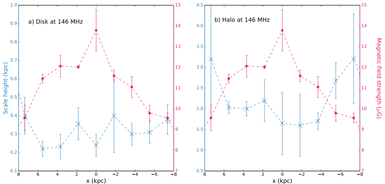
Fig. 16. Plot of the scale heights in kpc (dark blue) at 146 MHz and of the magnetic field strengths in \mu\text{G} (red) at different distances x from the galaxy’s centre along the major axis (in kpc). x > 0 corresponds to the north-eastern side of the galaxy and x < 0 to the south-western side. The disk scale heights are shown in the left panel, the halo scale heights in the right panel. The magnetic field strengths are measured from the 1.5 GHz data on the galaxy’s major axis and are identical in all four panels.
