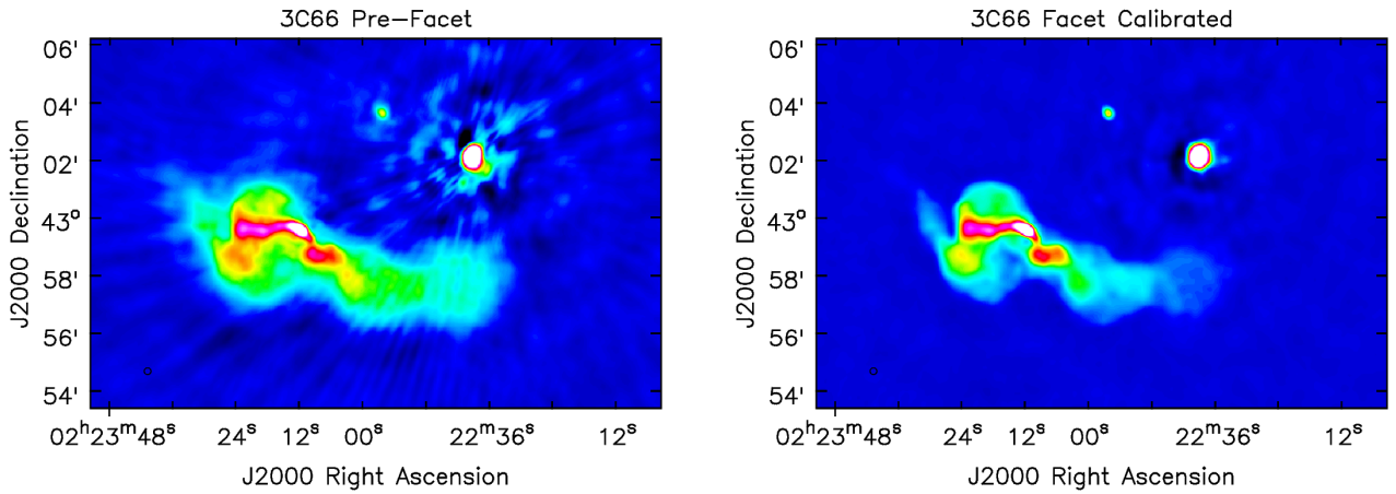
Fig. 1. Image of the compact source 3C66 A and the extended source 3C66 B after the initial direction-independent calibration (left) and after the direction-dependent facet calibration (right). Both images are smoothed to the same resolution of 14'' and are displayed on the same colour scale. The strong artefacts around 3C66 A after the direction-independent calibration in the left map are caused by the calibration not being adequate for this direction. After calibrating specifically for this direction these artefacts are mostly gone.
