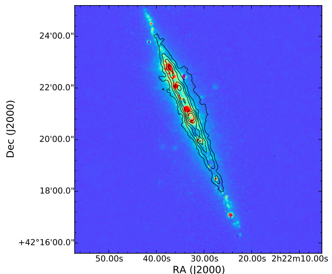
Fig. 6. H\alpha image of NGC 891 from Rand et al. (1990) (in colours) with the high resolution LOFAR image (Fig.3 left) overlaid as contours. Contours are at 12, 18, 25, 32, 44, 64 \times \sigma where \sigma = 0.29 mJy/beam is the rms noise level.
