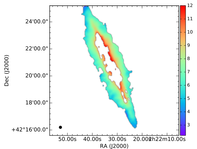
Fig. 12. Equipartition strength of the magnetic field B at 12'' resolution, in units of \mu\text{G} , determined by assuming energy equipartition between cosmic rays and magnetic fields. Pixels with \alpha_n > -0.6 are blanked. The beam is shown in the bottom left corner.
