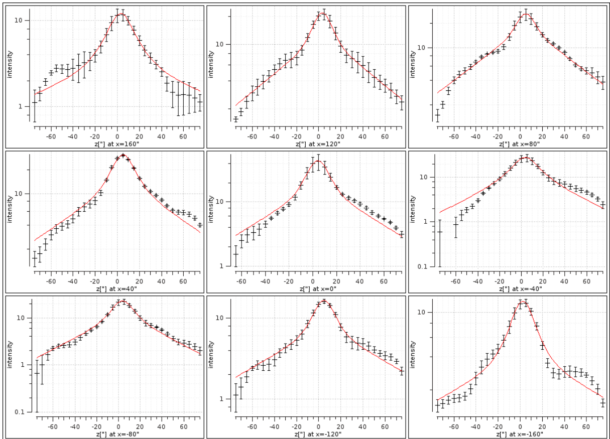
Fig. 14. Profiles of the average intensity at 146 MHz at 12'' resolution (in mJy/beam) as a function of distance z from the major axis (in arcseconds, 10'' \approx 0.46 kpc), for the 9 strips of NGC 891 at different distances, x , from the galaxy's centre along the major axis, corresponding to Fig. 13. The first panel is at x=+7.37 kpc (northern side), the last one at x=-7.37 kpc (southern side). z is negative (positive) on the eastern (western) side of the halo. The red lines show the two-component exponential functions fitted to the data.
