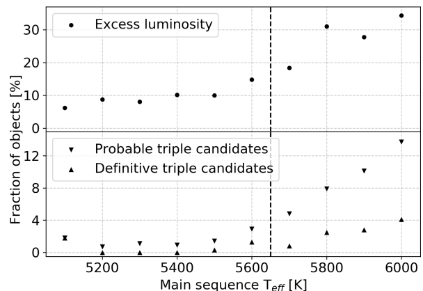
Figure 16. The upper panel shows the percentage of objects at different positions on the Kiel diagram shown in Figure 5 that show excessive luminosity and are spectroscopically similar to main sequence stars. Similarly, the lower panel shows upper and lower boundary on a percentage of triple system candidates at the same positions. For a definitive candidate, both fits must agree on a triple configuration. The strong dashed vertical line represents a point on Kiel diagram where the main sequence visually starts merging with the red-giant branch, the point where a region above the main sequence becomes polluted with more evolved stars.
