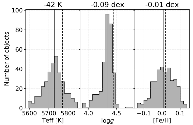
Figure 2. Distribution of physical parameters for discovered Solar twin candidates. Values above the plots represent difference between median of the distribution (solid vertical line) and actual Solar values (dashed vertical line).
