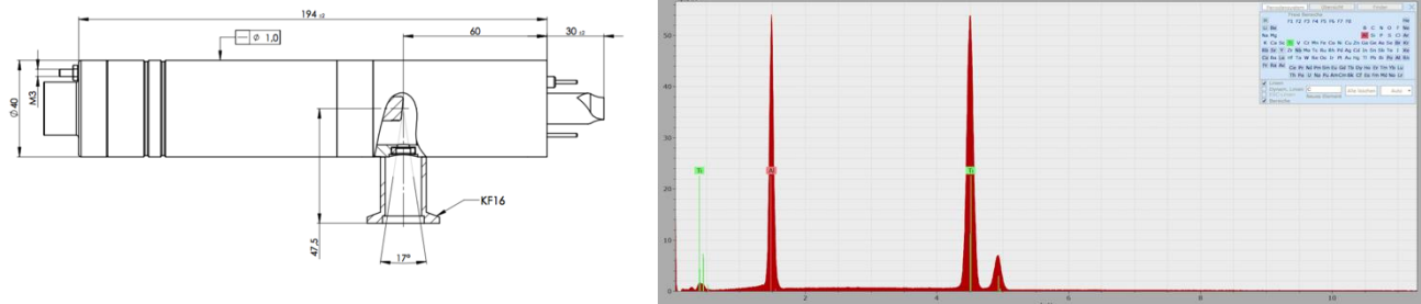
Figure 3: Left: scheme of the Incoatec X-ray microfocus source. Right: measured spectrum of the hybrid X-ray microfocus source with the anode in Ti-Al alloy (50% Al and 50% Ti), showing the X-ray fluorescence lines of both elements (courtesy by Incoatec).
