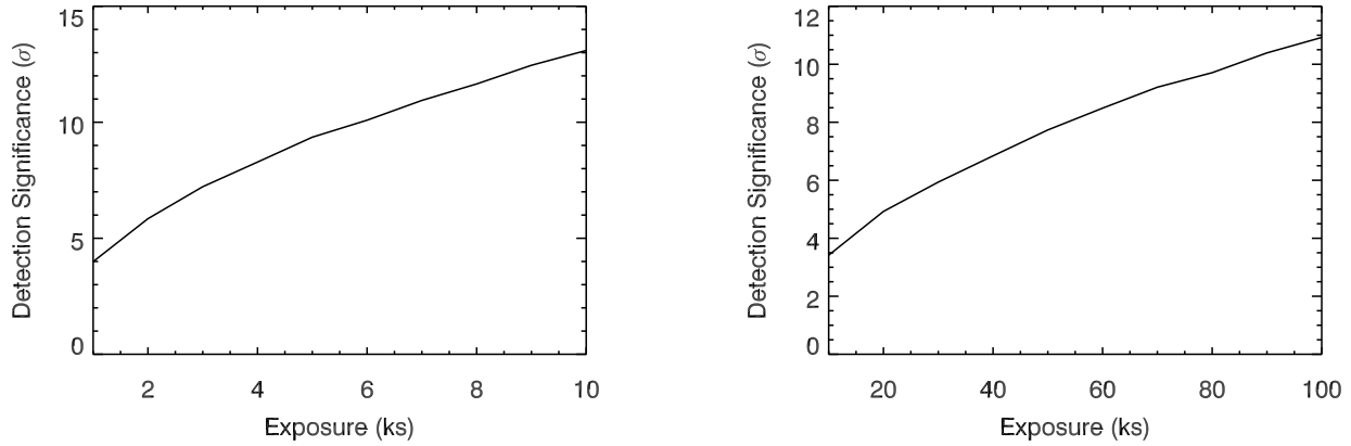
Figure 18 Simulations with eXTP showing the significance of a detection of a PF~70% (sufficient to prove QED effects) as a function of the exposure. Left: X-ray flux \sim 10^{-11} erg cm ^{-2} s ^{-1} , as typical of the outburst onset; Right: flux \sim 5 \times 10^{-13} erg cm ^{-2} s ^{-1} , as representative of the quiescent state after decay.
