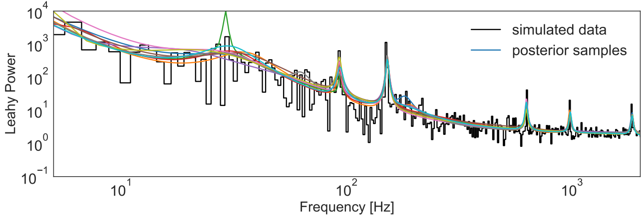
Figure 8 Black: simulated LAD eXTP data of the lightcurve of the IF observed from SGR 1900+14 in 2006, with quasi-periodic oscillations at 30 Hz, 92 Hz, 150 Hz, 625 Hz, 976 Hz, and 1840 Hz, at a fractional rms amplitude of 50% (with respect to that observed from the GF of SGR 1806–20). Overplotted in color are ten realizations from the posterior distribution of a mixture model of Lorentzian components, clearly identifying all but the lowest-frequency QPO present in the data.
