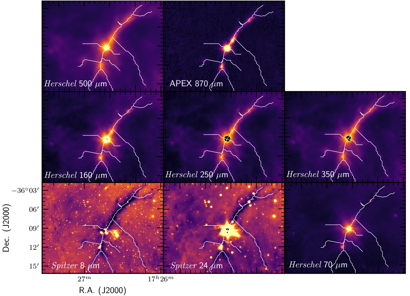
Fig. 2. Continuum images of G351 at different wavelengths from 8 \mu\text{m} with Spitzer (bottom left panel) to 870 \mu\text{m} with ATLASGAL-LABOCA. The LABOCA data are affected by filtering of large-scale emission (e.g. Schuller et al. 2009). The solid white line in each panel denotes the skeleton of G351 and of the branches.
