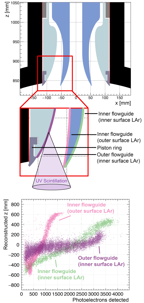
FIG. 18. Top & Middle: Cross-sectional illustration of the FG components in the AV neck. Shown are the three FG surfaces and the piston ring (not coated in LAr for purposes of illustration). Bottom: Simulated relationship in reconstructed z vs. PE for \alpha -decays on the IFG-IS (green), IFG-OS (pink), and OFG-IS (purple).
