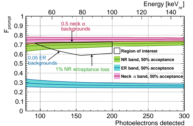
FIG. 20. Illustration of the WIMP ROI (black) along with the ER (blue), NR (green) and neck \alpha -decay (pink) bands that define the boundaries. Each band is drawn about the median of each class of event, with 25% of such signals above and 25% below included in the shaded regions.
