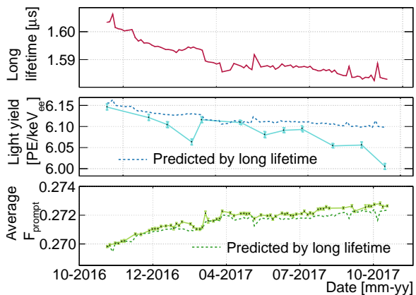
FIG. 13. Shown over the time period spanned by this dataset is the long lifetime component of LAr scintillation (top), the detector light yield (middle) and mean F_{\text{prompt}} of ER signals generated by 2.61 MeV \gamma -rays in the LAr target throughout the run. For the latter two plots, the predicted value based on the long lifetime value at that time is also shown (dashed).
