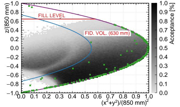
FIG. 23. Observed spatial distribution for all events surviving all cuts other than the cut on reconstructed radius. The color scale in the background shows the acceptance for ^{39}\text{Ar} events measured as a function of position after all but the radial cut; green points represent events in the ROI after all background rejection cuts. The fill level and radial fiducial cuts are drawn as well.
