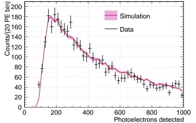
FIG. 6. Comparison of the detected PE distribution for high- F_{\text{prompt}} NR-like events from an AmBe neutron source simulation (pink) and data (black). The peak at low PE is due to the F_{\text{prompt}} cut that removed ERs; due to the high rate of ERs in coincidence with neutron-induced NRs in the calibration data, particularly strong cuts are needed to obtain a clean NR spectrum. Uncertainties shown are all statistical, using nominal values for the quenching and detector optics models.
