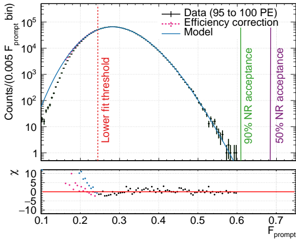
FIG. 7. F_{\text{prompt}} distribution for ERs from standard physics data in the lowest 1 keV ee energy bin in the WIMP-search region of interest. The PSD model is fit to the data to the right of the vertical dashed line, where the trigger efficiency is approximately unity. Agreement between the best fit model and the data can be seen; below the F_{\text{prompt}} fit region, trigger efficiency corrections to the data show that the model agrees when extrapolated to lower values. Solid vertical lines show the F_{\text{prompt}} value in the corresponding PE bins above which 90% or 50% of NRs are expected to be found. In the bottom plot, black points show residuals over the range where the model is fit; blue points compare the extrapolated model directly to the observed data prior to correcting for the decreasing trigger efficiency, while pink points compare the extrapolated model to the data after making these corrections.
