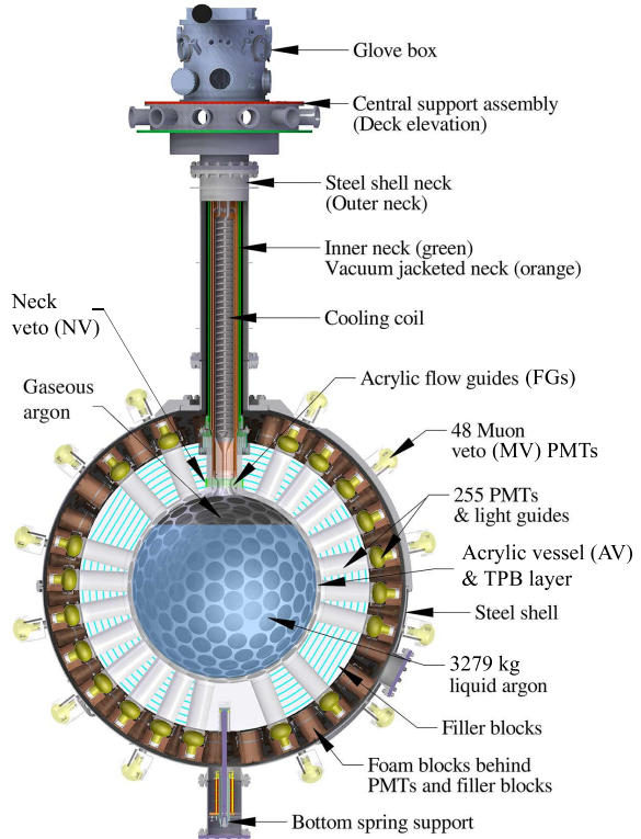
FIG. 1. Cross section of the DEAP-3600 detector components located inside the water tank (not shown). Inside the steel shell are inward-looking PMTs, light guides, filler blocks, and the acrylic vessel (AV), which holds the liquid argon target and the gaseous argon layer. Located on the outer surface of the steel shell are muon veto PMTs. Above this, a steel neck contains the neck of the AV, acrylic flowguides and the cooling coil. The neck is coupled to a central support assembly on which the glovebox is located. Shown also is the neck veto fiber system (green).
