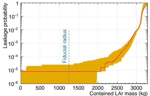
FIG. 17. Leakage probability for simulated \alpha -decays in the WIMP PE range vs. the contained LAr mass as determined by events within a given reconstructed radius. The contained LAr mass corresponding to the fiducial cut at 630 mm is shown. The systematic uncertainty on the probability is shown also (yellow band).
