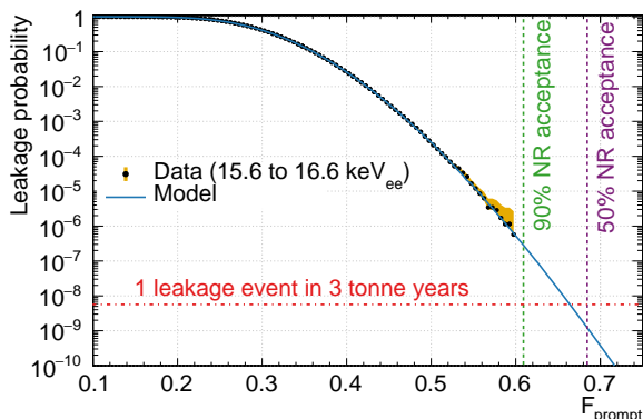
FIG. 14. Probability of an ER being detected above a given F_{\text{prompt}} value in the lowest 1 keV ee bin in the WIMP-search region of interest. For comparison, vertical lines show the values above which 90% or 50% of nuclear recoils are expected to be found.
