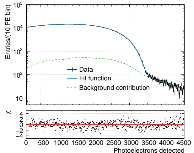
FIG. 4. ^{39}\text{Ar} model (blue line) fit to data (black). Included in the fit is the expected background contribution from \gamma -rays and ^{39}\text{Ar} pile-up events (green).
