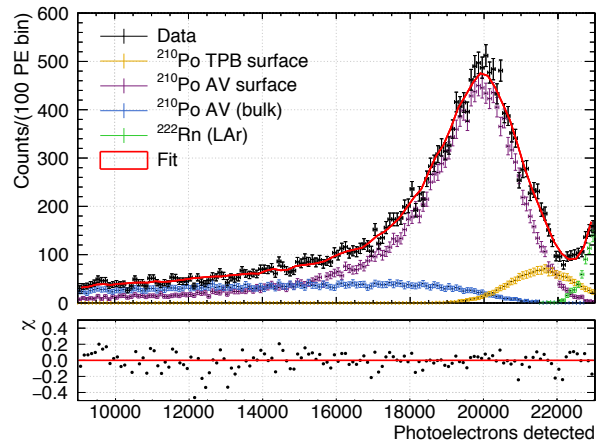
FIG. 16. PE distribution from data of ^{210}\text{Po} \alpha -decays candidates (black) alongside different simulated ^{210}\text{Po} samples located on the AV surface at the TPB/AV interface (purple), at the LAr/TPB interface and within the TPB layer (yellow) and from beneath the inner surface of the AV (blue). Shown also is the neighboring PE distribution from ^{222}\text{Rn} \alpha -decays in LAr (green). Overlaid is the combined fit (red) of each of these spectra to the observed PE spectrum from data. The event selections shown reconstruct with a z -position below the LAr fill level. No cut on the reconstructed radius is applied.
