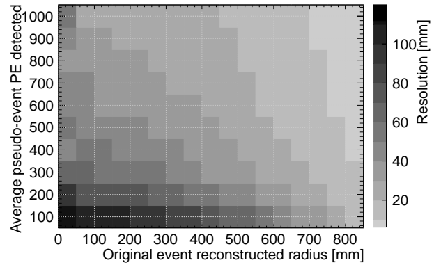
FIG. 11. Position resolution evaluated using the data-driven pseudo-event method, as a function of the average number of PE in both pseudo-events and the reconstructed radius drawn from the same original event, as returned by the PE-based algorithm. The z -axis scale denotes the resolution, defined as the characteristic width of the distribution of distances between reconstructed pseudo-events drawn from the same original event.
