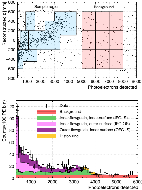
FIG. 19. Top: Distribution of reconstructed z vs. PE for events at high F_{\text{prompt}} in data, using the PE-based algorithm. Shown are trends from \alpha -decays in the neck between 300–5000 PE and a background sideband at higher PE values. The blue boxes denote the sample regions used by the template fit to compare with spectra from simulations. The red boxes are used to sample a background component. Bottom: 1D-projection of the observed PE spectra (black points) and expected distributions from the background model components, normalized to the best-fit rates.
