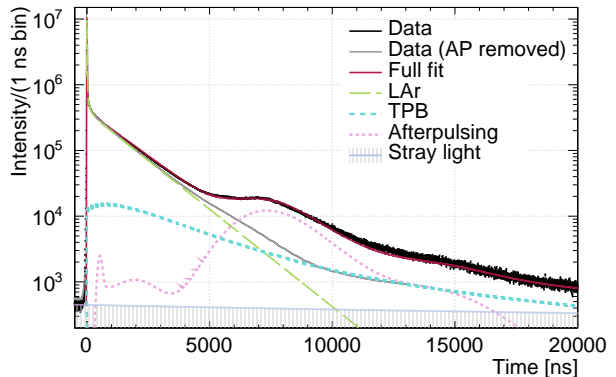
FIG. 3. Average ^{39}\text{Ar} pulseshape before correction of instrumental effects (black) shown together with a model fit (red). The fit accounts for the following effects, which are shown individually: LAr singlet, triplet, and intermediate [23] light emission (green dashed), TPB prompt and delayed light emission [24] (blue dash-dotted), afterpulsing following all the previous components (pink dotted), and stray light (grey filled), which accounts for dark noise and the delayed TPB emission from previous events. The pulse shape made from pulses that use the pulse-by-pulse AP removal algorithm (see text) is also shown (grey solid).
