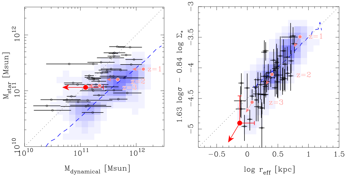
Figure 5. Left: stellar mass plotted against dynamical mass. The dotted line shows M_{\star} = M_{\text{dyn}} . The black points are the lower redshift objects ( z \sim 2 ) as in Figure 4. The shades are quiescent galaxies from LEGA-C, and the dashed curve is the running median of the distribution of quiescent galaxies with \text{sSFR} < 10^{-10} M_{\odot} \text{ yr}^{-1} drawn from SDSS DR15 (Aguado et al. 2019). SFR and stellar mass are from Granada FSPS fits (Ahn et al. 2014). The red point is the z = 4 object. The pink points are the expected evolutionary track assuming constant velocity dispersion (see the text for details). Right: mass fundamental plane. The dotted line is a fit from Bezanson et al. (2013). The other symbols are the same as those in the left panel.
