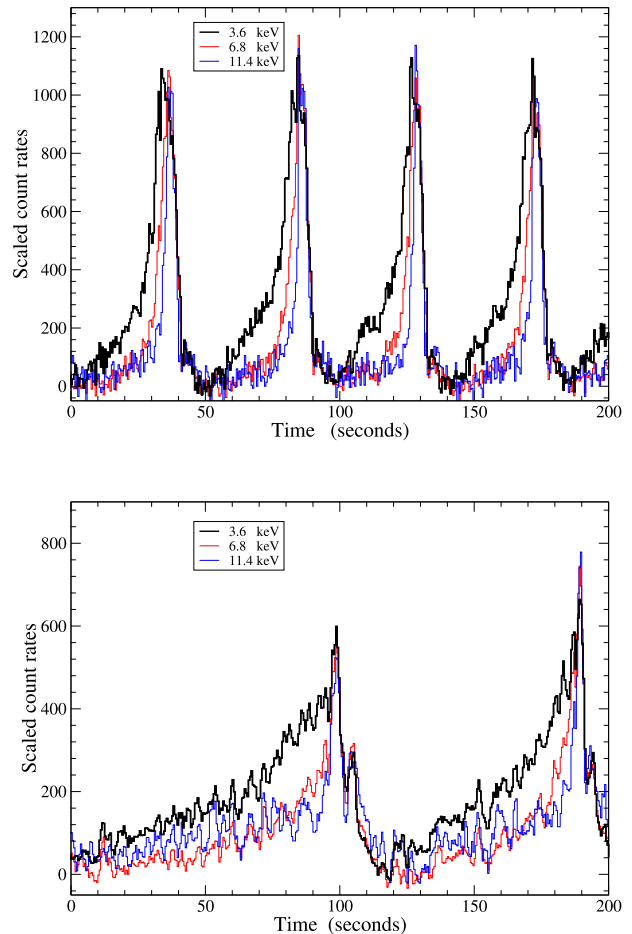
Fig. 1. Two segments of RXTE/PCA light curves of GRS 1915+105 in the \rho variability class at three energies showing the HXD phenomenon and the dependence of the pulse width, w , upon energy. Data, after the subtraction of a constant level, are scaled to obtain comparable pulse heights. Upper panel: RXTE G-2a data; lower panel: G-1 data. In the latter data set the recurrence time of the bursts was more than twice longer than that in the former one. We note in both panels the variable duration and shape of individual bursts and in the upper one the small time delay of the peak maxima, particularly in the first and in the third burst.
