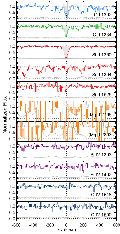
Figure 69. Stacked velocity plot for the z = 5.8987 system toward ATLAS J158-14. Lines and shading are as described in Figure 11. The gray histogram in the O I \lambda 1302 panel is the deblended flux. See notes on this system in Appendix B.
