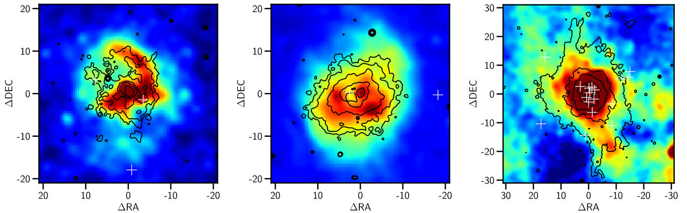
Figure 10. Chandra images of NGC 5846, NGC 4636, and NGC 5044 with superimposed contours of their respective H\alpha + [N II] emission. An excellent correlation is apparent in the central region, as well as in the extended filamentary structures of the three galaxies. White crosses mark the detected CO cloud positions.
