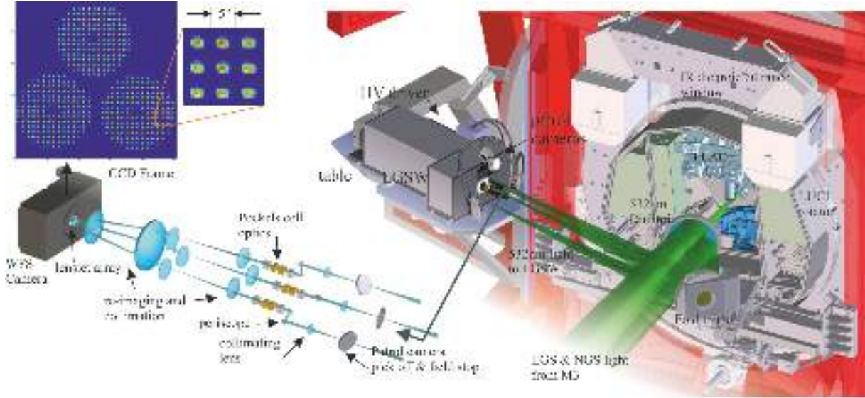
Fig. 7. Optical path and CAD model of one of the wavefront sensors. The light from the LGSs enters from the right side in its 4 arcmin wide constellation. Patrol cameras enable a fast acquisition and position control of the guide stars. Inside the wavefront sensor units motorized mirrors stabilize the field and the pupil, driven by the signals from the WFS CCD. After that the gating units slice out the photon bunches originating from the 12 km distant scattering, letting a 300 m range (i.e. 2 \mu\text{s} ) long part pass to the wavefront sensor detector. These Pockels cells units operate at the same 10 kHz as the laser pulses are sent to sky. The wavefront sensor detector accumulates the charge originating from 10 consecutive pulses, being read out at a 1 kHz frame rate. The wavefront sensor CCD frame of one telescope side with the three LGSs is shown on the left. Having passed a common microlens array in front of the detector, all three guide stars show a Shack–Hartmann spot pattern on the detector. From each spot the local wavefront slope can be measured, enabling the reconstruction and correction of the ground-layer turbulence. Because LGS spots are often larger than NGSs, the sub-aperture’s field of view amounts to \sim 5'' sampled with 8 \times 8 pixels on the CCD frame.
