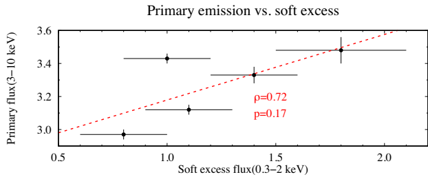
Figure 11. The primary X-ray flux (3–10 keV) of the hot N_{\text{THCOMP}} component versus the flux (0.3–2 keV) of the warm N_{\text{THCOMP}} component, as measured in the different observations. The fluxes are in units of 10^{-11} ergs \text{s}^{-1} \text{cm}^{-2} . The red dashed line represents a linear fit to the data.
