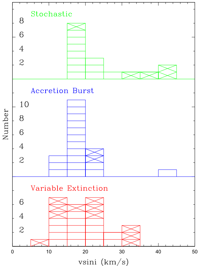
Figure 14. Histogram of estimates of the projected rotational velocity derived from Gaussian fits to the Li I 6708 Å doublet for the variable extinction, accretion burst, and stochastic light curve classes. Stars with spectral type K3 or earlier are marked with a cross; not unexpectedly, these stars include most of the rapidly rotating CTTS in the three classes.
