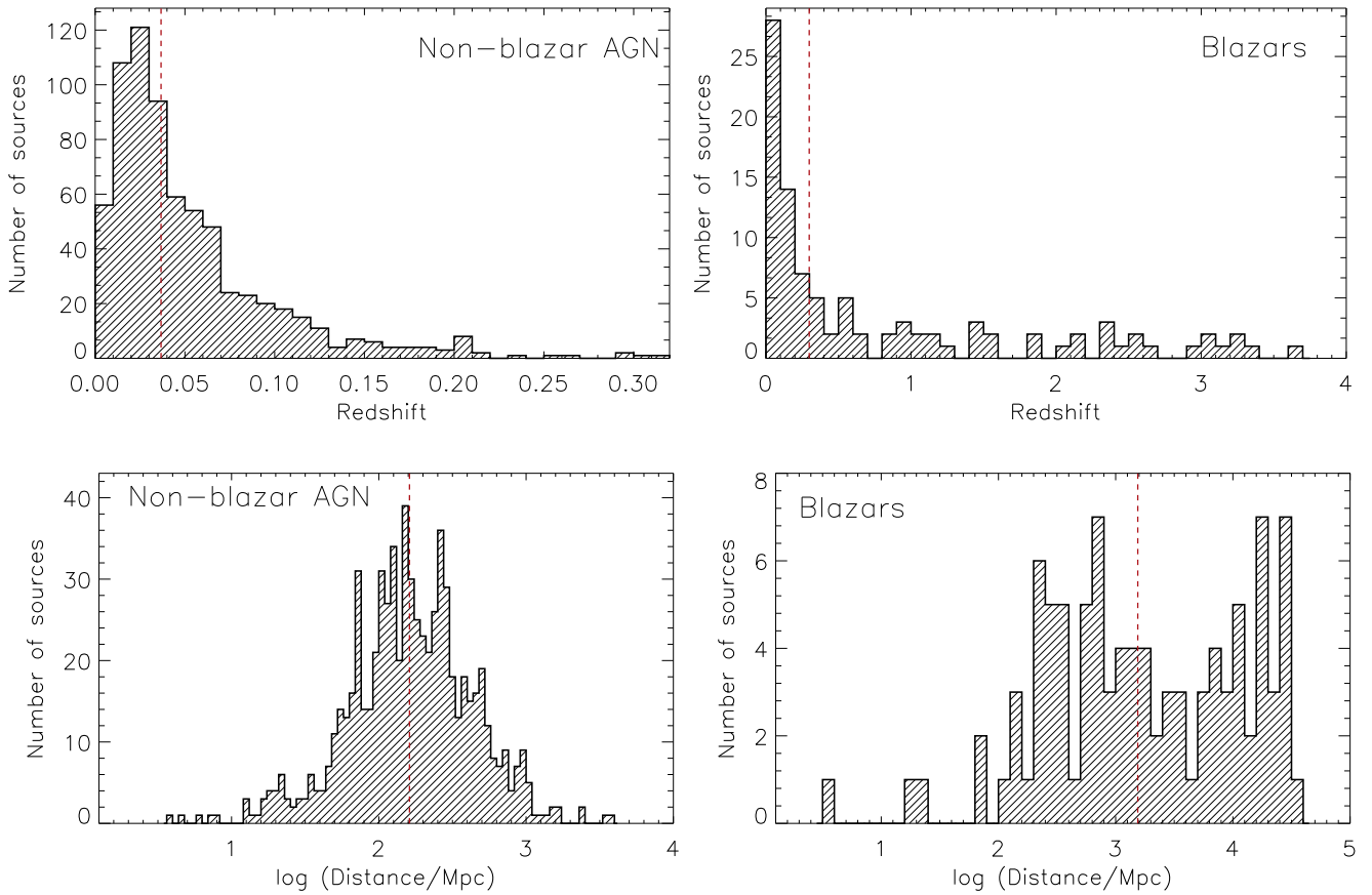
Figure 2. Top left panel: zoom-in of the z = 0 – 0.32 range of the redshift distribution of the nonblazar AGNs of our sample. There are four nonblazar AGNs at z \geq 0.4 that are excluded from this plot: SWIFT J1131.9–1233 ( z = 0.6540 ), SWIFT J2344.6–4246 ( z = 0.5975 ), SWIFT J1159.7–2002 ( z = 0.4500 ), and SWIFT J0216.3+5128 ( z = 0.422 ). Top right panel: redshift distribution of the blazars. Bottom left panel: distribution of the distances of the nonblazar AGNs of our sample (including the redshift-independent distances). Bottom right panel: same as the bottom left panel, but for the blazars. For all panels the red dashed lines show the median for each sample. Among the 70-month catalog sources, nonblazar AGNs lie at much lower redshifts and distances (median values: z = 0.0367 , D = 161.6 Mpc) compared to the strongly beamed and more luminous (see Section 5.1 and Figure 14) blazar population ( z = 0.299 , D = 1565.3 Mpc).
