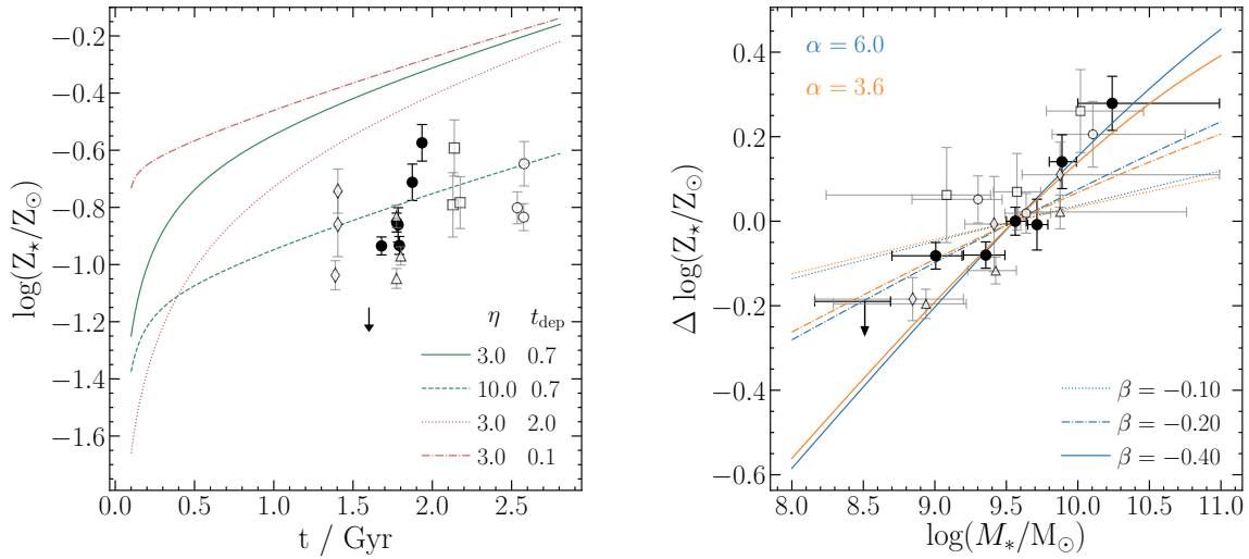
Figure 12. The evolution of \log(Z_*/Z_\odot) as a function of cosmological time (left-hand plot) and \Delta\log(Z_*/Z_\odot) as a function of stellar mass (right-hand plot) compared to predictions from the one-zone analytic chemical evolution models of Weinberg et al. (2017). The left-hand plot shows the time evolution of \log(Z_*/Z_\odot) from t = 0 (i.e. the Big Bang) to the age of the Universe at the minimum redshift of our sample ( z = 2.3 ; t = 2.8 Gyr). The green curves show \log(Z_*/Z_\odot) evolution assuming a constant depletion timescale ( t_{\text{dep}} = 0.7 Gyr) for two different values of the mass-loading parameter ( \eta = 3 and 10 ) while the maroon curves show the evolution assuming a fixed value of \eta = 3.0 and two different values of the depletion timescale ( t_{\text{dep}} = 0.1 and 2 Gyr). The significantly sub-solar abundances of our sample ( \sim 10 - 20\% ) require mass outflow rates roughly an order of magnitude greater than the star formation rates (averaged across all stellar masses). The right-hand plot shows the difference in \log(Z_*/Z_\odot) as a function of stellar mass assuming different forms of the M_* - \eta relationship. The functional form is taken from the scaling relation presented by Muratov et al. (2015) (see Eq. 5). The orange and blue lines show the \Delta\log(Z_*/Z_\odot) - \log(M_*/M_\odot) predictions relative to the value at \log(M_*/M_\odot) \simeq 9.5 for different assumptions of the absolute mass-loading parameter at that stellar mass; \eta = 3.6 and \eta = 6 (see text for discussion). Regardless of the normalization, the evolution of \log(Z_*/Z_\odot) as a function of stellar mass is consistent with a power law exponent \beta < -0.2 and in good agreement with the Muratov et al. (2015) result ( \beta = -0.36 ).
