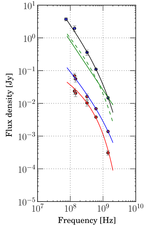
Fig. 7. JP and KGJP model fits for Regions 4 (blue) and 16 (red), along with the corresponding data points (LOFAR HBA, GMRT, and VLA). The sum of the fits for all regions is represented by the dashed green line. The integrated flux density data points (VLSS, LOFAR HBA, GMRT, and VLA) are best fitted by a KGJP model (black line) with an injection index of \alpha_0 = -1.23 \pm 0.37 and t_{\text{on}} = 0.1 Myr, t_{\text{off}} = 77.7 Myr. The measurement regions do not cover the source completely at lower frequencies, so the sum of the fits does not precisely follow the integrated flux density. A CI model that is rejected by the integrated flux data is represented with a green line.
