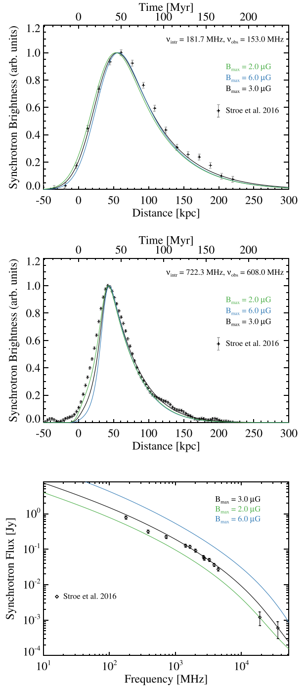
Figure C2. Beam convolved brightness profiles at 150 MHz and 610 MHz and integrated synchrotron spectrum (top to bottom) for the exponential model with minimum magnetic field B_{\max} equal to 3 \mu\text{G} (standard model, black), 2 \mu\text{G} (green) and 6 \mu\text{G} (blue).
