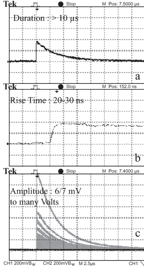
Figure 3: Typical signal from the Big Pad on a 50 \Omega load. The signal is reported in a) with a horizontal scale of 2.5 \mu s and in b) with a horizontal scale of 100 ns. In both cases the vertical scale is 10 mV. In Fig.3c the vertical scale is 200 mV (horizontal scale 2.5 \mu s) with the oscilloscope set at infinite persistence and triggered for 20 minutes by particles crossing the chamber.
