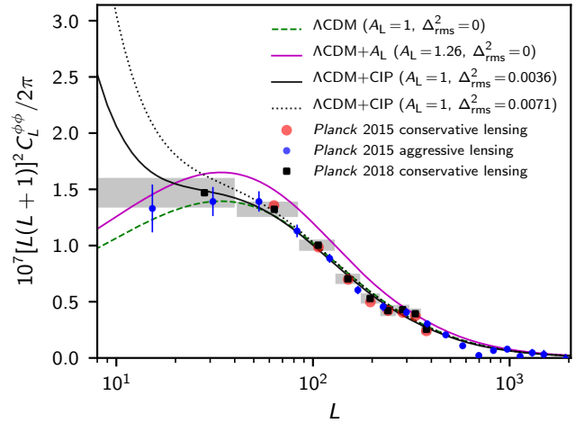
Fig. 46. Conservative Planck 2015 lensing data (red points), aggressive Planck 2015 lensing data (blue points with error bars), and conservative Planck 2018 lensing data (black squares in grey boxes), along with the best-fit models to the Planck data: the best-fit adiabatic \Lambda CDM model to 2018 TT +lowE (green dashed line); the best-fit \Lambda CDM+ A_L model to 2018 TT +lowE (magenta solid line, A_L = 1.26 ); and the best-fit \Lambda CDM+CIP model to 2018 TT, TE, EE +lowE and conservative lensing data (black solid line, \Delta_{\text{rms}}^2 = 0.0036 ) and to 2015 TT, TE, EE +lowP and conservative lensing data (black dotted line, \Delta_{\text{rms}}^2 = 0.0071 ). As CIP modifies only the very low- L part of the lensing power spectrum, the conservative 2015 lensing data ( 40 \leq L \leq 400 ) are insensitive to CIP even when \Delta_{\text{rms}}^2 = 0.0071 . On the other hand, the first two data points of the 2015 aggressive lensing data disfavour the large CIP amplitude ( Smith et al. 2017 ), which gives a very good fit to all the other data. Planck 2018 conservative lensing data cover the range 8 \leq L \leq 400 and consequently disfavour CIP variances \Delta_{\text{rms}}^2 \gtrsim 0.004 .
