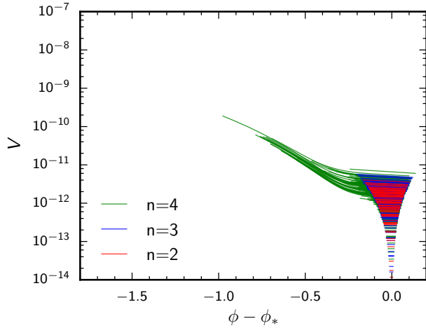
Fig. 12. Representative sample of the observable region of inflaton potentials allowed at the 95% CL, when the potential is Taylor-expanded at order n = 2, 3, and 4 in the observable region, making no assumption about the end of inflation, and using Planck TT,TE,EE+lowE+lensing+BK15. In natural units (where \sqrt{8\pi}M_{\text{Pl}} = 1 ). We use the same scales as in PCI15. Note that there is another branch of solutions that is symmetric under (\phi - \phi_*) \rightarrow -(\phi - \phi_*) .
