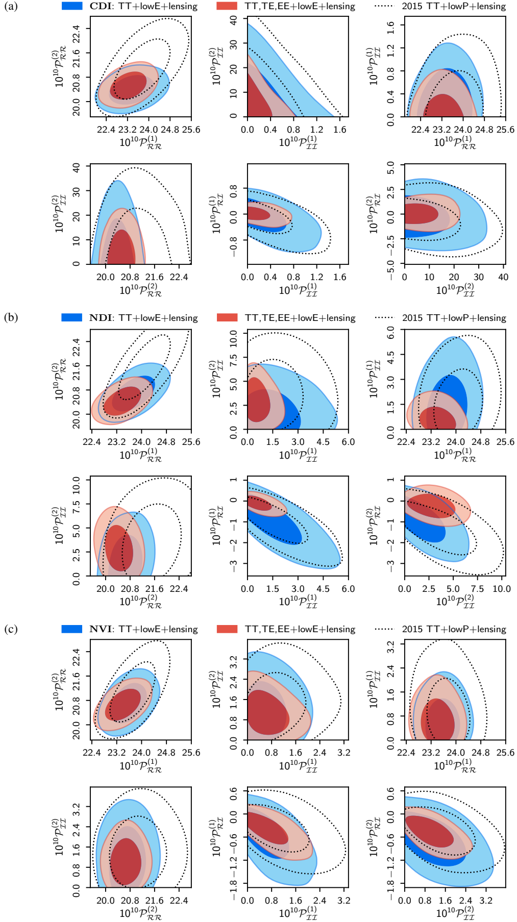
Fig. 38. Constraints on the primordial perturbation power in generally correlated ADI+CDI (a), ADI+NDI (b), and ADI+NVI (c) models at two scales, k_1 = 0.002 \text{ Mpc}^{-1} (1) and k_2 = 0.100 \text{ Mpc}^{-1} (2). Note that in our modelling \mathcal{P}_{\mathcal{R}\mathcal{I}}^{(2)} is not an independent parameter.
