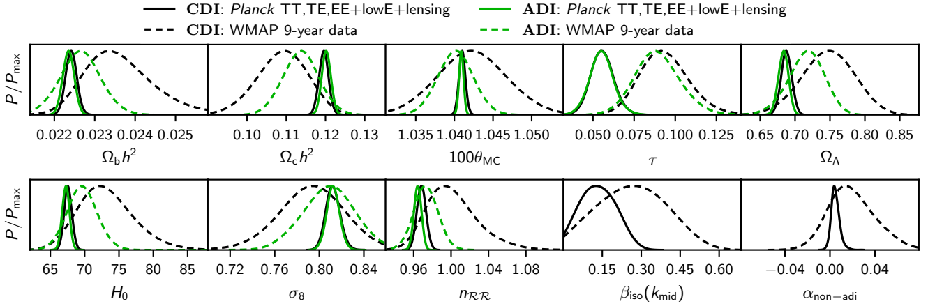
Fig. 42. Comparison of posterior probability density for selected cosmological parameters with Planck data and pre- Planck (i.e., WMAP 9-year) data. Black lines indicate the results obtained for the generally correlated mixed CDI+ADI model, and green lines for the pure adiabatic model.
