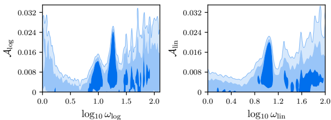
Fig. 28. Marginalized joint 68%, 95%, and 99% CL regions of the modulation amplitude versus frequency parameter using the TT,TE,EE data set for the logarithmic (left) and linear (right) oscillation models.
