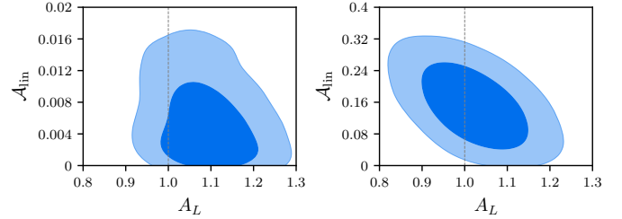
Fig. 29. Marginalized joint 68% and 95% CL regions for the lensing parameter A_L and the modulation amplitude parameter \mathcal{A}_{\text{lin}} using the TT data set. Left: Linear oscillation model with \log_{10} \omega_{\text{lin}} = 1.158 and \varphi_{\text{lin}} = \pi . Right: Modified linear oscillation model with a Gaussian envelope function (see text) and \log_{10} \omega_{\text{lin}} = 1.158 , \varphi_{\text{lin}} = \pi , \mu_{\text{env}} = 0.2 \text{ Mpc}^{-1} , and \sigma_{\text{env}} = 0.057 \text{ Mpc}^{-1} .
