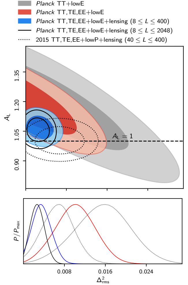
Fig. 47. Degeneracy between A_L and \Delta_{\text{rms}}^2 in the \Lambda CDM+ A_L +CIP model (top panel) and constraints on \Delta_{\text{rms}}^2 in the \Lambda CDM+CIP model, where A_L = 1 (bottom panel).
