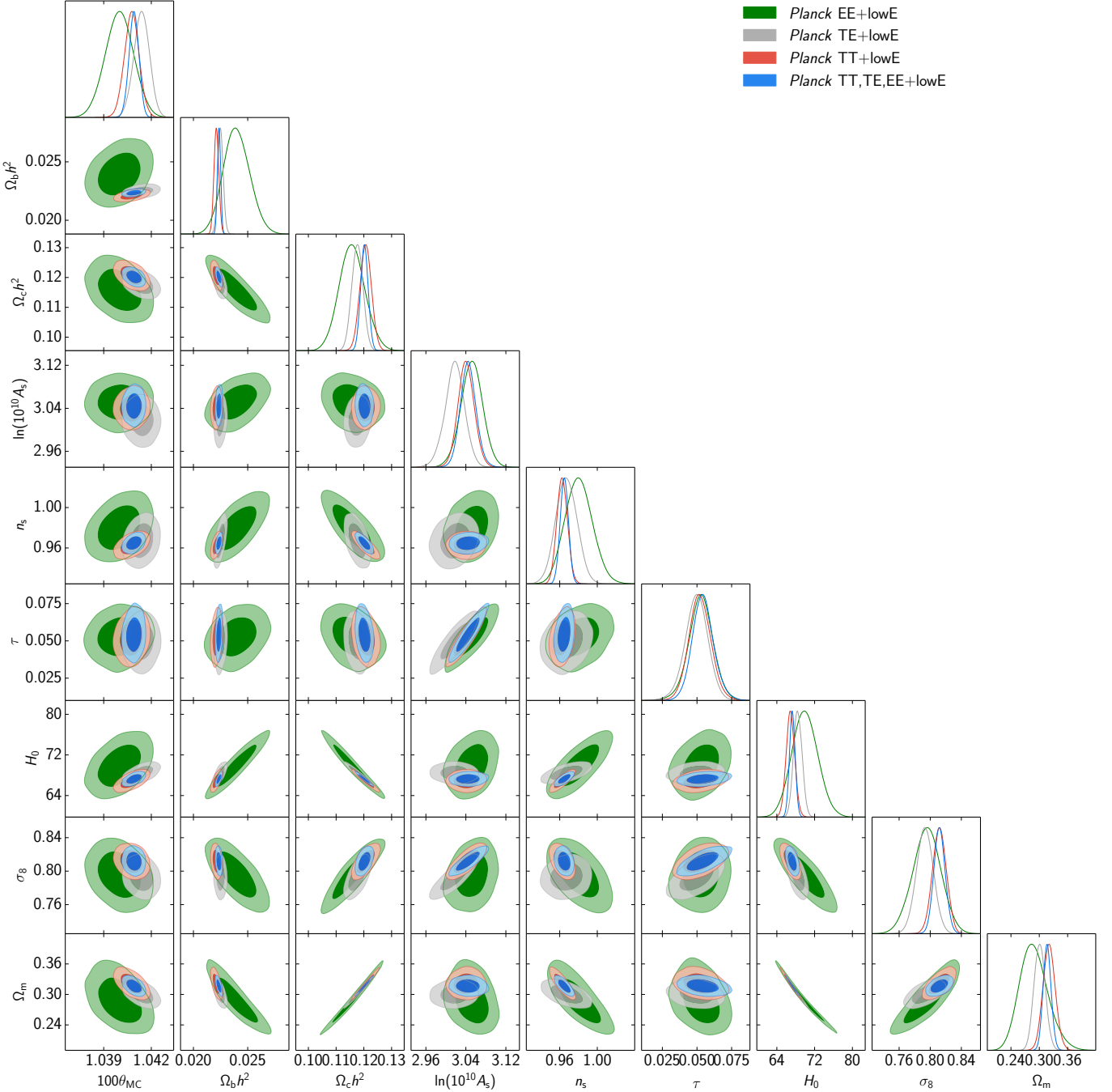
Fig. 2. Marginalized joint 68 % and 95 % CL regions for the cosmological parameters in \Lambda CDM with Planck TT, EE, TE, and joint TT,TE,EE, all in combination with the EE likelihood at low multipoles.
