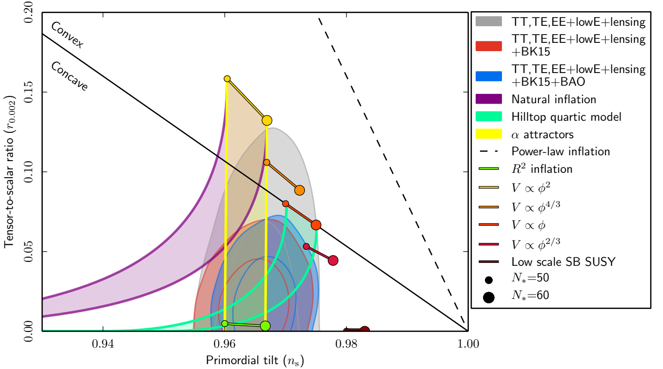
Fig. 8. Marginalized joint 68 % and 95 % CL regions for n_s and r at k = 0.002 \text{ Mpc}^{-1} from Planck alone and in combination with BK15 or BK15+BAO data, compared to the theoretical predictions of selected inflationary models. Note that the marginalized joint 68 % and 95 % CL regions assume dn_s/d \ln k = 0 .
