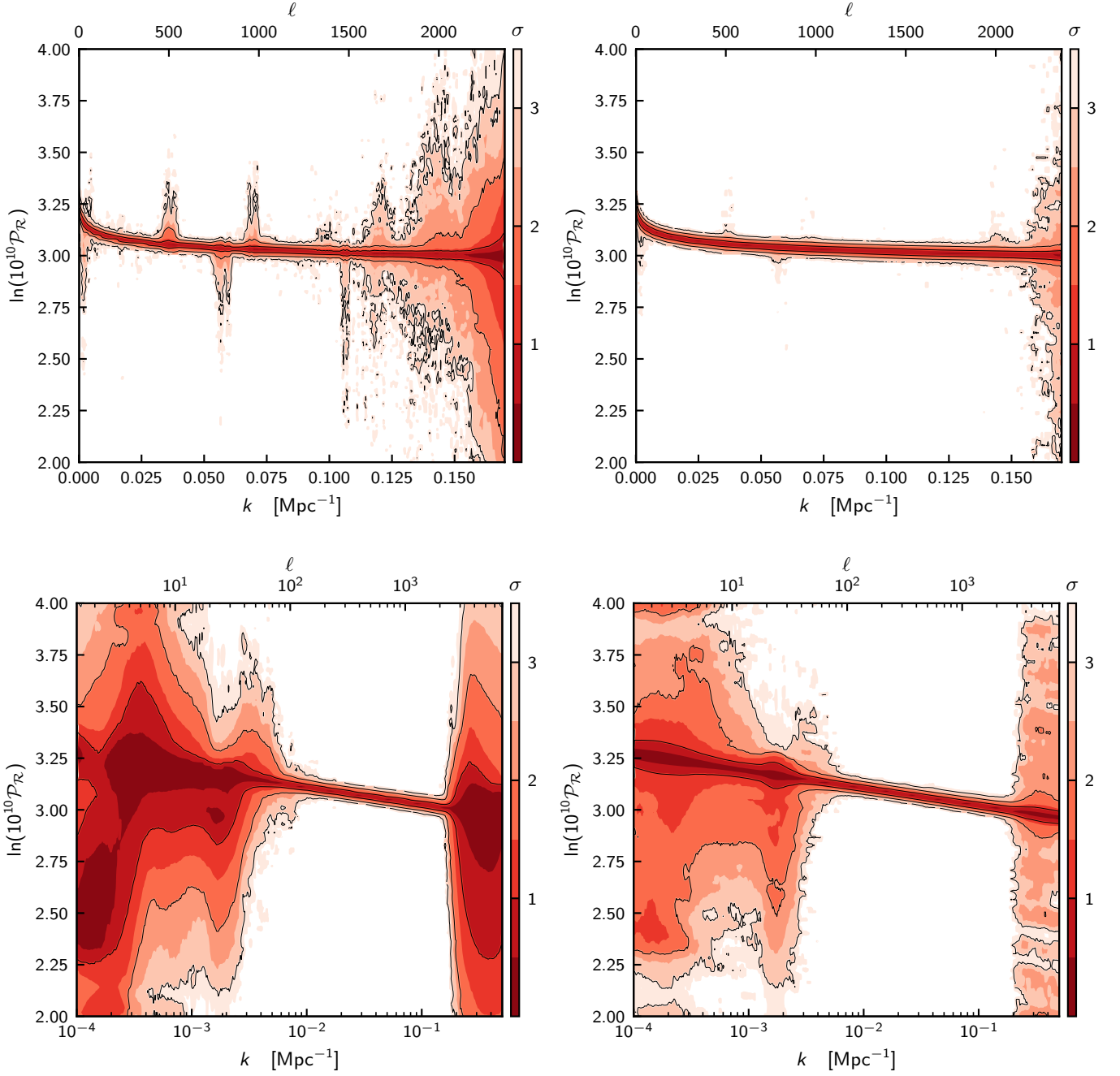
Fig. 22. Free-form Bayesian search for features (Sect. 6.2.2) with Planck TT,TE,EE+lowE+lensing. The upper panels show runs with linear priors on the k -locations. The lower panels use logarithmic priors on the k -features. Left panels show the reconstruction for N = 8 features, while the right panels show the reconstruction marginalized over N = 0, \dots, 8 features.
