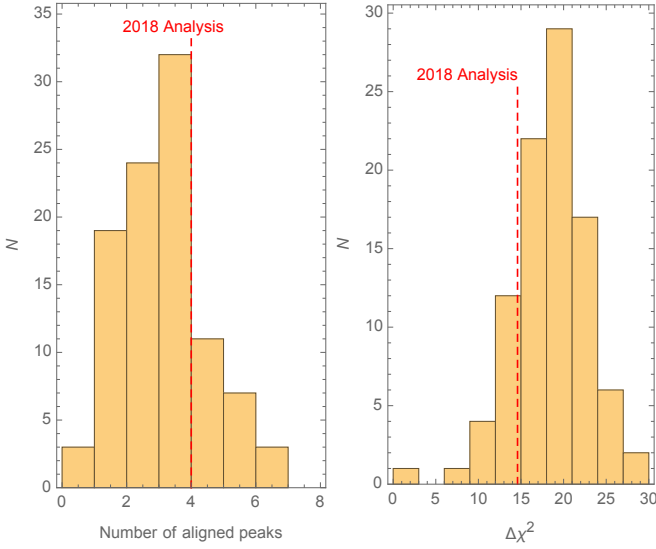
Fig. 36. Left: Number of aligned peaks in the power spectrum and the bispectrum for the log feature model. Right: Mean improvement of those same peaks in 100 simulated bispectra combined with the unbinned high- \ell likelihood.
