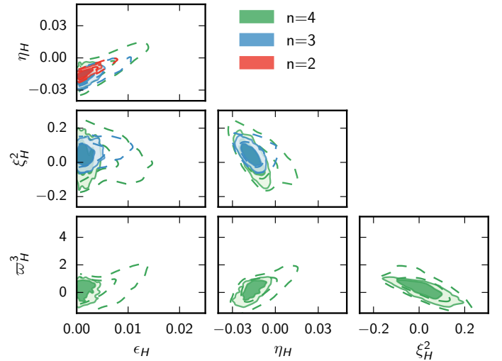
Fig. 13. Taylor expansion of H(\phi) at order n = 2, 3, and 4 in the observable region, making no assumption about the end of inflation. The parameters are combinations of Taylor coefficients with flat priors. Dashed contours are Planck TT,TE,EE+lowE, while solid contours are Planck TT,TE,EE+lowE+lensing+BK15. The scales are the same as in PCI15.
