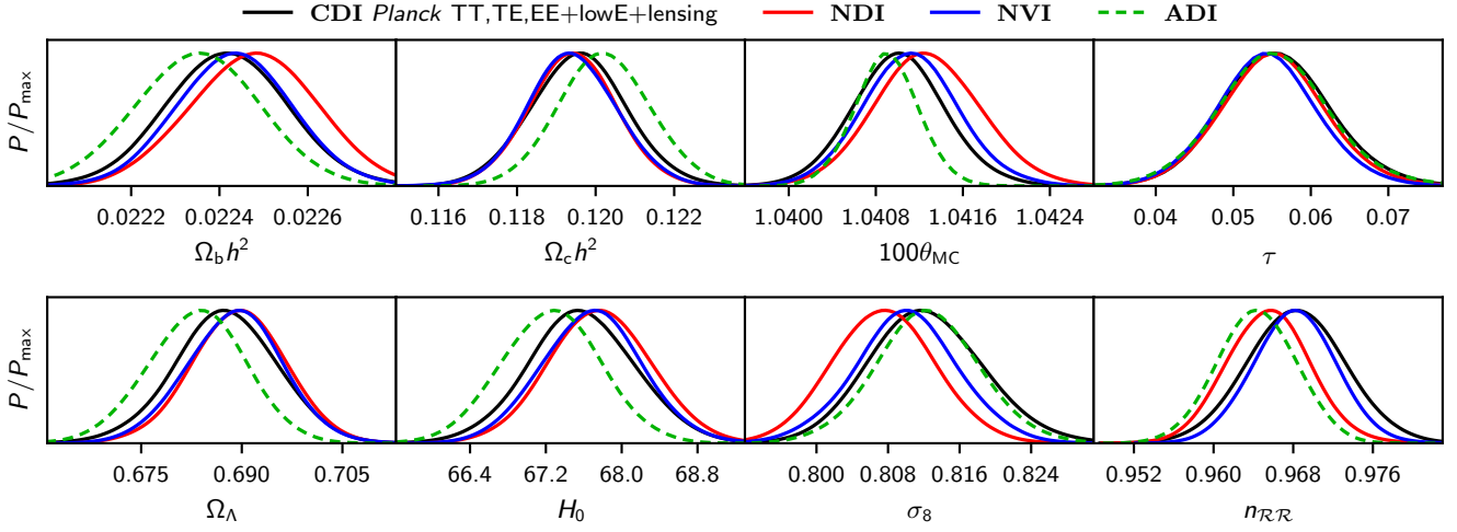
Fig. 41. Comparison of posterior probability density for the standard cosmological parameters in mixed adiabatic and isocurvature models (solid lines) to those in pure adiabatic \Lambda CDM model (ADI, dashed green lines), using Planck TT,TE,EE+lowE+lensing data.
