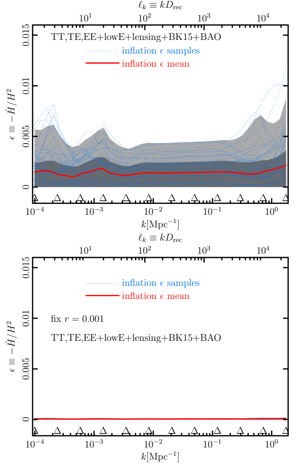
Fig. 26. Acceleration history \epsilon(k) for reconstructed trajectories using 12 knots (marked as \Delta at the bottom of the figure), with cubic-spline interpolation and the Planck TT, TE, EE+lowE+lensing+BK15+BAO data for the two cases of floating r and r fixed at 0.001. Sample 1\sigma trajectories for the floating r case allow wide variability, which is naturally greatly diminished if r is fixed to r = 0.001 .
