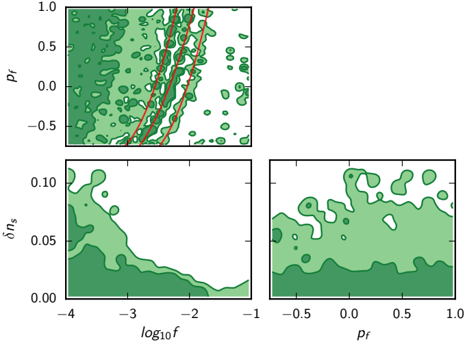
Fig. 33. Same as Fig. 32, but for the case of p = 1 .
