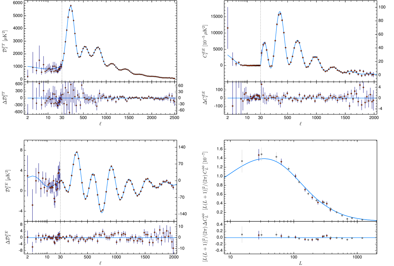
Fig. 1. Planck 2018 CMB angular power spectra, compared with the base- \Lambda CDM best fit to the Planck TT,TE,EE+lowE+lensing data (blue curves). For each panel we also show the residuals with respect to this baseline best fit. Plotted are \mathcal{D}_\ell = \ell(\ell+1)C_\ell/(2\pi) for TT and TE , C_\ell for EE , and L^2(L+1)^2 C_L^{\phi\phi}/(2\pi) for lensing. For TT , TE , and EE , the multipole range 2 \leq \ell \leq 29 shows the power spectra from Commander ( TT ) and SimAll ( TE , EE ), while at \ell \geq 30 we display the co-added frequency spectra computed from the Plik cross-half-mission likelihood, with foreground and other nuisance parameters fixed to their best-fit values in the base- \Lambda CDM cosmology. For the Planck lensing potential angular power spectrum, we show the conservative (orange dots; used in the likelihood) and aggressive (grey dots) cases. Note some of the different horizontal and vertical scales on either side of \ell = 30 for the temperature and polarization spectra and residuals.
