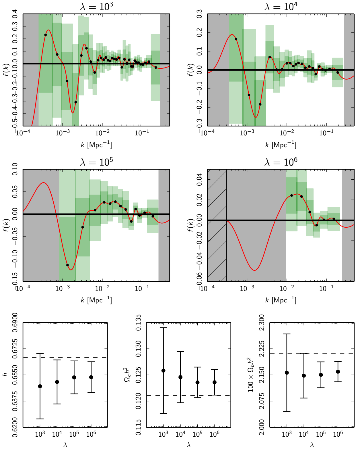
Fig. 18. Planck TT+lowE penalized likelihood primordial power spectrum reconstruction. Top four panels: The deviation f(k) for four different roughness penalties. The red curves indicate the best-fit deviation, while the vertical extents of the dark and light green error bars indicate the \pm 1\sigma and \pm 2\sigma errors, respectively. The width of the error bars indicates the minimum reconstructible width (the minimum width for a Gaussian feature such that the mean square deviation of the reconstruction is less than 10%). The grey regions display where the minimum reconstructible width is undefined, meaning that the reconstruction in these regions is untrustworthy. The hatched region in the \lambda = 10^6 plot indicates where the fixing penalty has been applied. Lower three panels: \pm 1\sigma error bars for the three non-primordial-spectrum cosmological parameters included in the reconstruction. The respective best-fit fiducial model values are indicated by the dashed lines.
