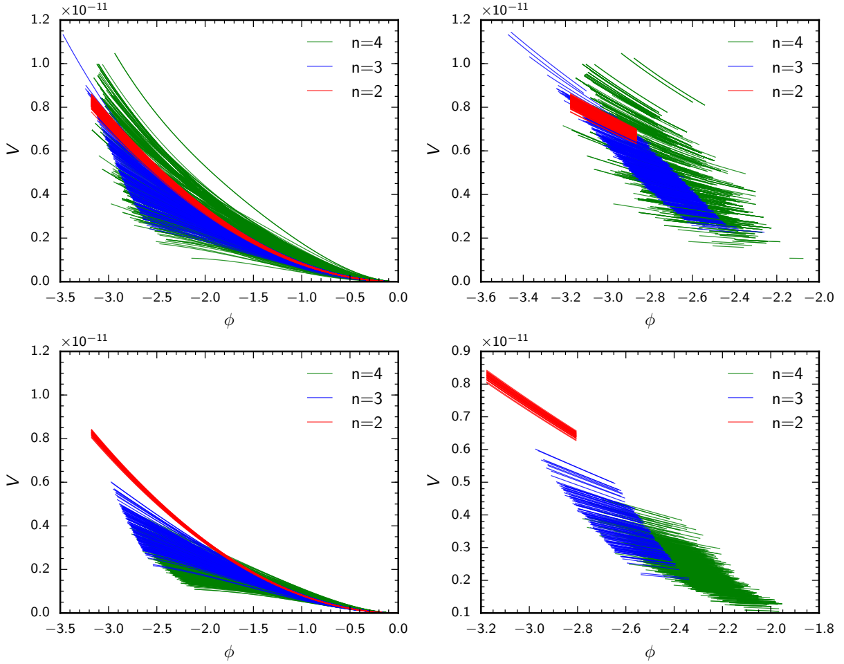
Fig. 16. Representative sample of the inflaton potentials allowed at the 95 % CL, when the potential is Taylor-expanded at order n = 2, 3 , and 4 and trusted until the end of inflation, and under the assumption of N_* = 55 e -folds of inflation between Hubble-radius crossing for the pivot scale and the end of inflation. In natural units (where \sqrt{8\pi M_{\text{Pl}}} = 1 ). Left panels: Full potential from the beginning of the observable window till the end of inflation. Right: Zoom on the observable window directly constrained by inflation. Top: Planck TT,TE,EE+lowE. Bottom: Planck TT,TE,EE+lowE+lensing+BK15. Note that there is another branch of solutions that is symmetric under \phi \rightarrow -\phi .
