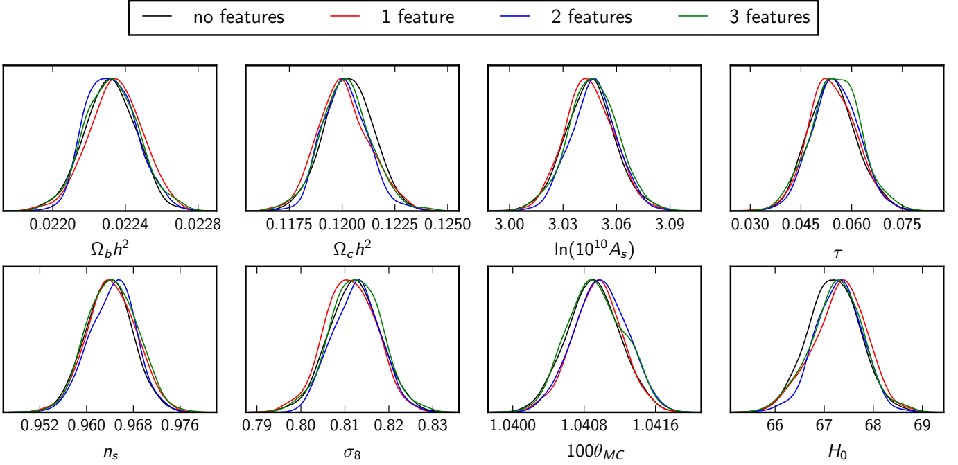
Fig. 23. The effect on the underlying cosmological parameters of the free-form Bayesian search for features (Sect. 6.2.2), for N = 0, \dots, 3 features with linear k -priors. The parameters remain stable up to N = 8 features, and when changing to logarithmic k -priors.
