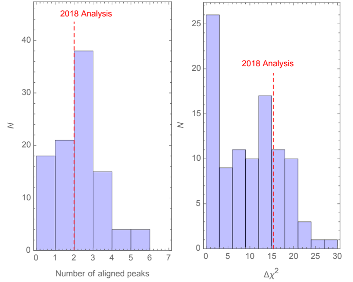
Fig. 37. Left: Number of aligned peaks in the power spectrum and the bispectrum for the linear feature model. Right: Mean improvement of those same peaks in 100 simulated bispectra combined with the unbinned high- \ell likelihood.
