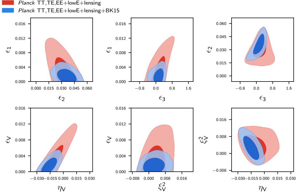
Fig. 7. Marginalized joint two-dimensional 68 % and 95 % CL regions for combinations of (\epsilon_1, \epsilon_2, \epsilon_3) (upper panels) and (\epsilon_V, \eta_V, \xi_V^2) (lower panels) for Planck TT,TE,EE+lowE+lensing (red contours), compared with Planck TT,TE,EE+lowE+lensing+BK15 (blue contours).
