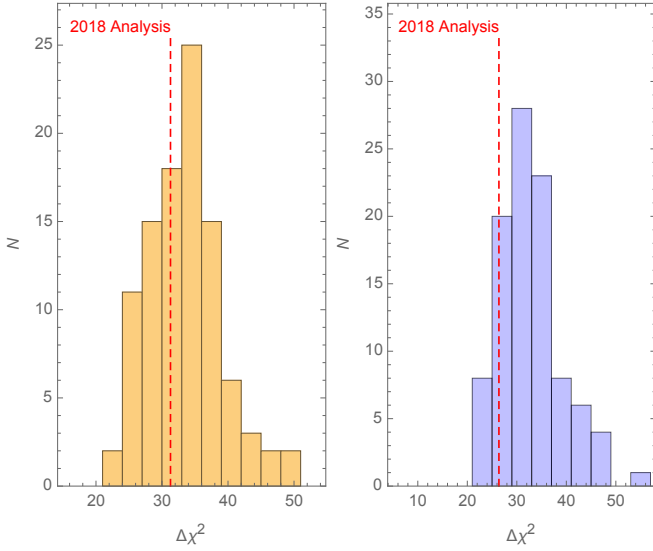
Fig. 35. Typical best-fit improvement in units of \Delta\chi^2 in 100 simulations compared to the real data (red dashed lines) for the log feature (left) and the linear feature (right) models.
