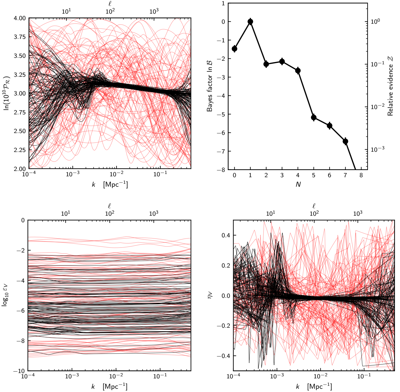
Fig. 17. Free-form potential reconstructions using Planck TT+TE+EE+lowl+lowE+lensing (Sect. 5.4). The top-right panel shows Bayes factors for the free-form potential reconstruction. The preferred reconstruction has N = 1 , corresponding to a constant non-zero d^2 \ln V_1 / d\phi^2 . The remaining panels show reconstructions for the N = 8 knot case, focusing on the scalar primordial power spectrum, and the inflationary slow-roll parameters \epsilon_V and \eta_V . Red lines indicate sample trajectories from the prior, whilst black lines are from the posterior. Technically the slow-roll parameters are defined as functions of \phi , but we instead substitute this for the Hubble-radius-exit value to make for clearer comparison between posterior samples. In all plots, the approximate link between \ell and k is via the Limber approximation, \ell \simeq k/D_A , where D_A = r_*/\theta_* is the comoving angular distance to recombination, which is at comoving distance r_* .
