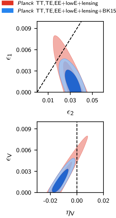
Fig. 6. Marginalized joint two-dimensional 68 % and 95 % CL regions for (\epsilon_1, \epsilon_2) (top panel) and (\epsilon_V, \eta_V) (bottom panel) for Planck TT,TE,EE+lowE+lensing (red contours), compared with Planck TT,TE,EE+lowE+lensing+BK15 (blue contours). The dashed lines divide between convex and concave potentials.
