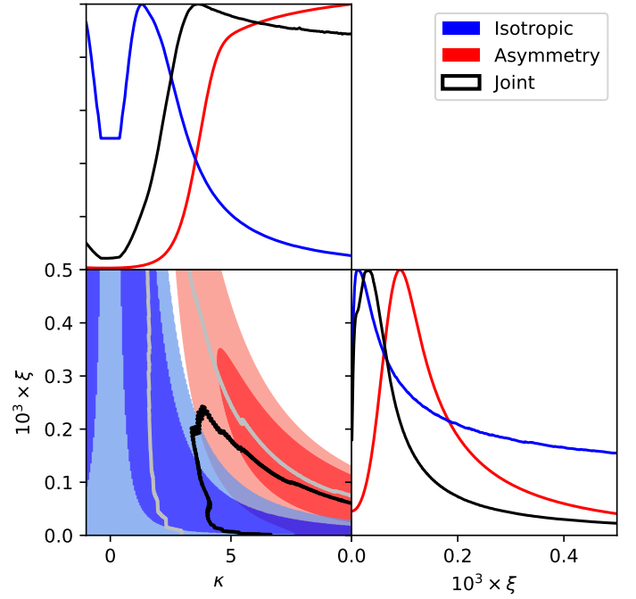
Fig. 48. Posteriors for the curvaton dipolar modulation model parameters \kappa and \xi . Contours enclose 68 % and 95 % of the posteriors. The model can explain the well-known dipolar asymmetry: note the preference for \xi > 0 in the asymmetry constraint (red contours and curves). However, the modulation preferred by the asymmetry constraint is reduced substantially when the isotropic constraint (blue) is added (black). The asymmetry constraint here uses SMICA, while the isotropic constraint uses Planck TT,TE,EE+lowE+lensing. Resolution is reduced at very small \kappa due to the sampling in \beta_{\text{iso}} .
