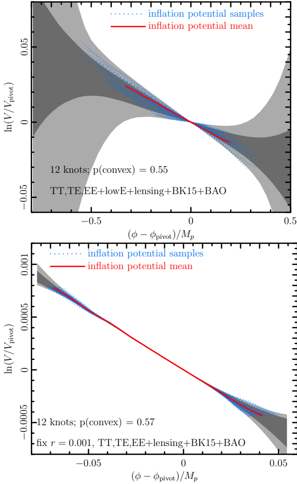
Fig. 27. Top: Reconstructed shape of the single-field inflaton potential from the cubic-spline power spectra mode-expansion using 12 knots and the Planck TT,TE,EE+lowE+lensing+BK15+BAO data. Bottom: Result when r is fixed at 0.001. Instead of plotting as a function of wavenumber k we plot \ln V(\phi)/V_{\text{pivot}} about a pivot field value \phi_{\text{pivot}} . Note that the range on the \phi axis is quite different for the small r case than the floating case. The probability of local convexity evaluated at \phi_{\text{pivot}} is denoted as p(\text{convex}) .
