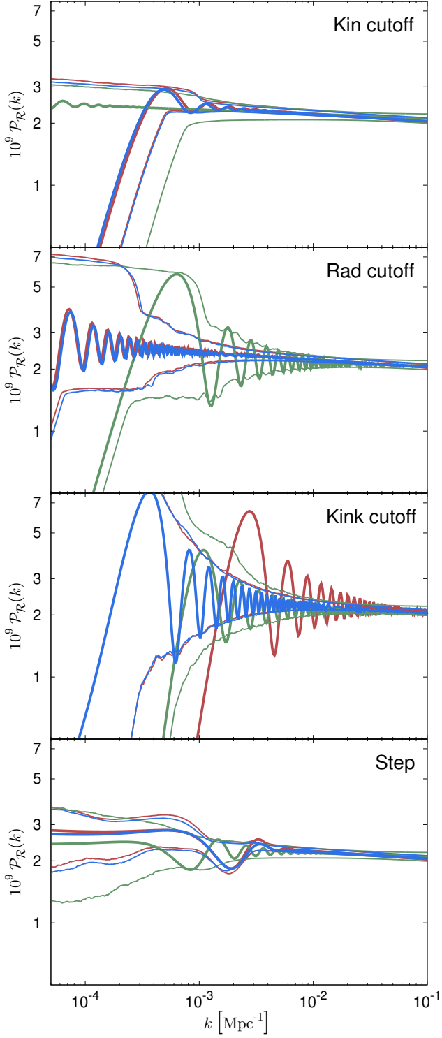
Fig. 30. Best-fit and central 95 % CL regions for the primordial power spectrum in the three cutoff and the step models for TT data (red curves), EE data (green), and TT,TE,EE data (blue). Note that for the combination of kink cutoff model and TT data, the best-fit value for the cutoff scale k_{\text{kink}}^c lies close to the prior boundary, and therefore the best-fit spectrum does not fall within the central 95 %-credible band.
