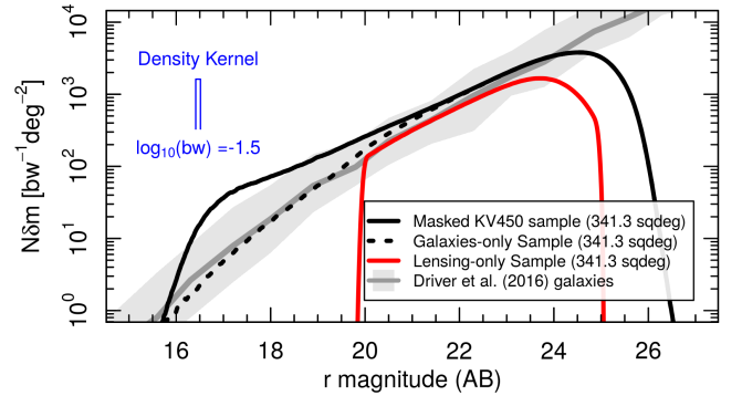
Fig. 6. r -band number counts for sources in KV450 before ( solid black ) and after ( dotted black ) removal of stars, and for the lensing sample ( red ). Each of these datasets is presented as raw number density; i.e. the number counts divided by the area of the sample (indicated in the legend), without any additional weighting. We compare these to the galaxy number counts from the literature compendium presented in Driver et al. (2016). The grey region shows the scatter in the data from their literature compendium, while the solid grey line traces the median of their compendium. Our number counts are in good agreement with the literature. At the bright end our hot-mode source extraction leads to a dearth of the brightest galaxies (causing the dashed black line to begin to fall downwards at magnitudes brighter than r \sim 19.5 ).
