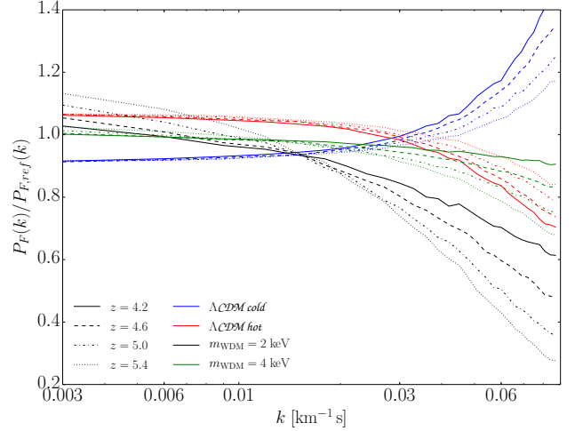
FIG. B.5: The flux power spectrum for different models varying mass of the WDM ( m_{\text{WDM}} ) and the amplitude of the IGM temperature at the mean density ( T_0^A ). The colours show two values of m_{\text{WDM}} - 2 keV in black and 4 keV in green - and two \Lambda\text{CDM} models with different temperatures - hot IGM in red (roughly 3000K hotter) and cold in blue (roughly 3000K colder). The reference model against which the flux power is compared, was \Lambda\text{CDM} model with T_0(z = 3.6) = 11000\text{K} . Different line styles show the redshift evolution of the flux power: full line ( z = 4.0 ), dashed line ( z = 4.6 ), dot-dashed line ( z = 5.0 ) and dotted line ( z = 5.4 ). As with Fig. B.2, only the effect on the largest redshift bins is shown since that is where the effect of WDM on the smoothing scale becomes largest.
