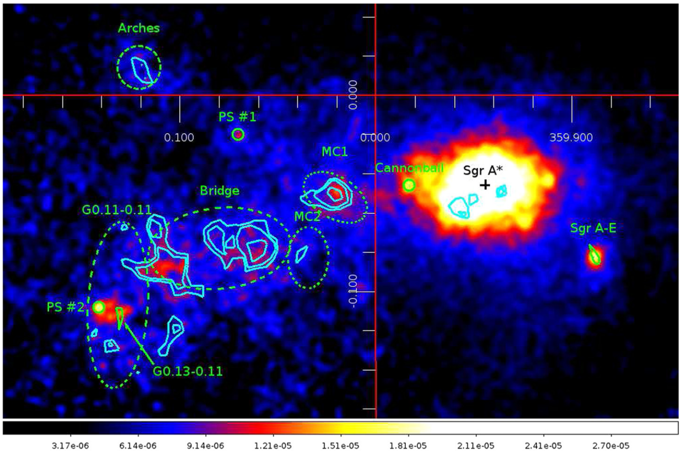
Figure 3. NuSTAR 10–20 keV exposure-corrected smoothed image of the GC region in the Galactic coordinates [°]. Green dashed ellipses: selected molecular clouds. Cyan contours: 6.4 keV Fe K- \alpha continuum-subtracted intensity contours from XMM-Newton . Green polygons: Chandra morphologies of the two X-ray filaments detected above 10 keV. Green circles ( r = 10'' ): two hard X-ray point sources. PS #1 and #2 are known Chandra point sources, CXOUGC J174551.9–285311 and CXOUGC J174622.7–285218, respectively (Muno et al. 2009).
