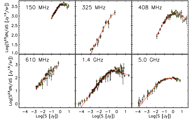
Figure A1. Comparison of our best-fit evolutionary model for RL AGNs with Euclidean normalized differential counts at several frequencies. Data points are from the compilation by De Zotti et al. (2010) . As is well known, AGNs become sub-dominant compared to SFGs at sub-mJy flux density levels.
