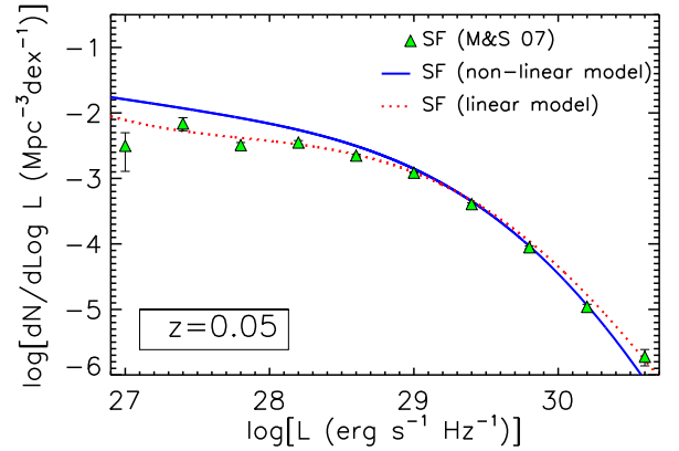
Figure 1. Comparison between the observational determination of the local RLF of SFGs at 1.4 GHz (data points; Mauch & Sadler 2007 ) and the one obtained from the local SFR function using either eq. (4) with a dispersion of 0.4 dex (dotted red curve) or eq. (5) with a dispersion of 0.3 dex (solid blue line).
