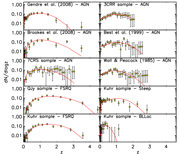
Figure A2. Comparison of our best-fit evolutionary model for RL AGNs with observational determinations of the redshift distributions for several source samples. See Massardi et al. (2010) for a description of the samples and for references.
