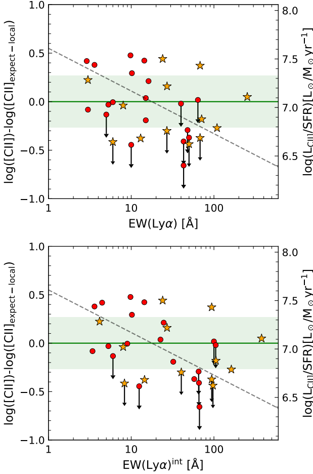
Figure 7. Top panel: Offset from the local L_{\text{CII}}\text{-SFR} relation as a function of \text{EW}(\text{Ly}\alpha) . The right hand axis shows the L_{\text{CII}}/\text{SFR} ratio corresponding to the deviations from the local L_{\text{CII}}\text{-SFR} relation. The 1\sigma dispersion of the local relation is indicated by the shaded green region. Star and circles indicate sub-components and individual galaxies, respectively. The grey dashed relationship shows our linear fit (see text). Bottom panel: Same as the top panel but the \text{EW}(\text{Ly}\alpha)^{\text{int}} has been corrected for the IGM absorption by following Harikane et al. 2017.
