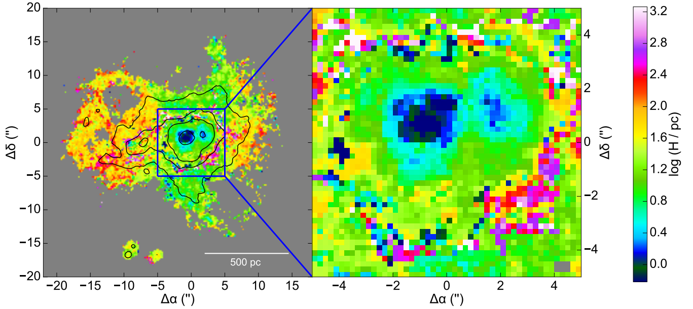
Figure 4. Left panel: “effective” scale height defined as H = N_H/n . As in Fig. 1, black lines show the contours of the H\alpha emission line (80, 10, 4, and 1 in units of 10^{-16} ergs s^{-1} cm^{-2} ). Right panel: zoom on the blue box.
