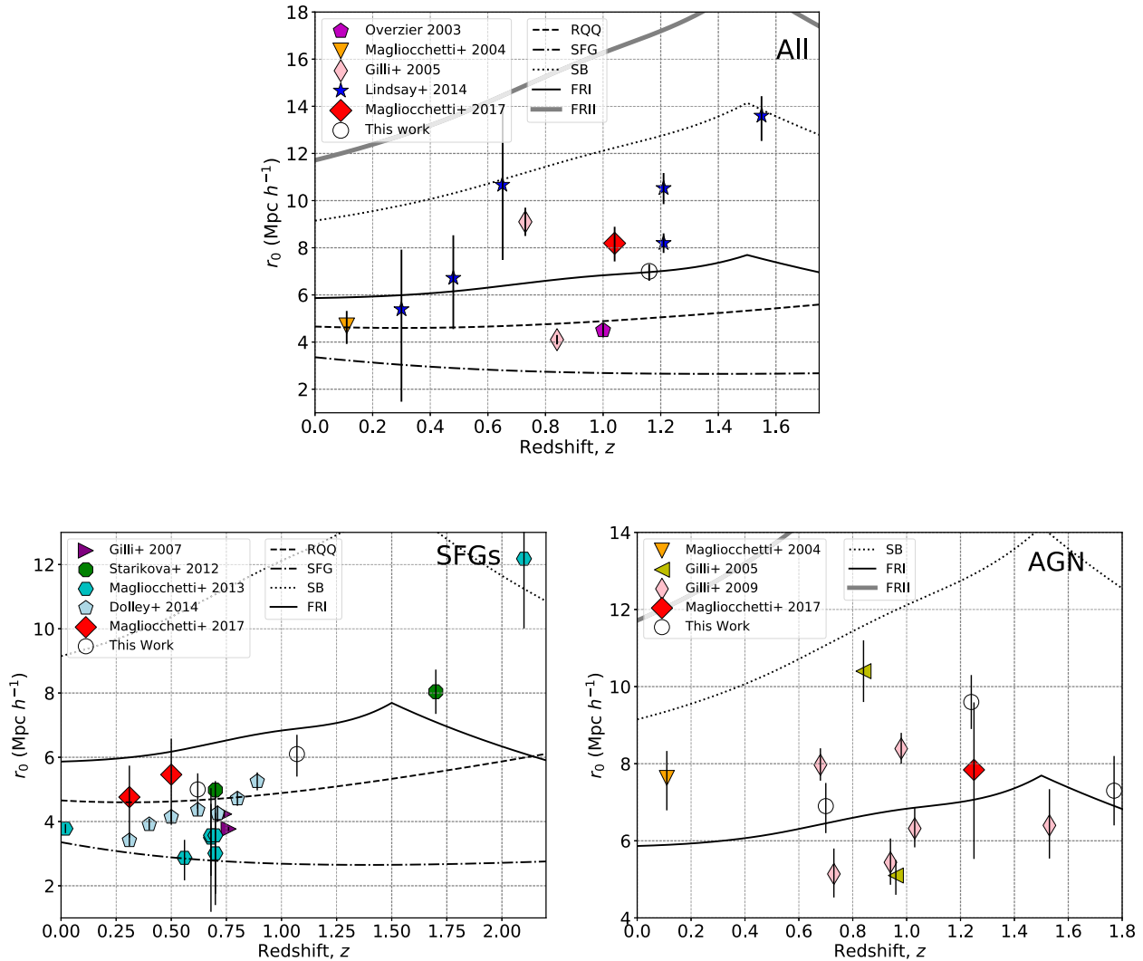
Figure 9. Comparison of our r_0 values (open circles) to previous studies for: all galaxies (top); SFGs (bottom left); and AGN (bottom right). These are for all z , z < 1 , and z \geq 1 where appropriate. Previous work is from: Overzier et al. (2003) (magenta pentagon); Magliocchetti et al. (2004) (orange downwards triangles); Gilli et al. (2005) (yellow left triangles – for the Chandra Deep Field-North and Chandra Deep Field-South fields); Gilli et al. (2007) (purple right triangles – for the GOODS-North and GOODS-South fields); Gilli et al. (2009) (pink thin diamonds – for: all AGN; all AGN with a spike in galaxies at z \sim 0.36 removed; z < 1 AGN; z < 1 AGN with a spike in galaxies at z \sim 0.36 removed; AGN with z \geq 1 ); Starikova et al. (2012) (green octagon); Magliocchetti et al. (2013) (cyan hexagons – showing points for IRAS galaxies; the COSMOS field; Extended Groth Strip ; GOODS-South field); Lindsay et al. (2014a) (blue stars); Dolley et al. (2014) (pale blue pentagons – over a range of redshifts); and Magliocchetti et al. (2017) (red diamonds). This is adapted from fig. 4 in Magliocchetti et al. (2017). For all studies shown, the redshifts presented are the median redshift of the sample, however, the samples will span a large range in redshifts, which is not shown. The lines show the evolution of r_0 as expected from Wilman et al. (2008) for: radio-quiet quasars (RQQ, dashed); star-forming galaxies (SFG, dot-dashed); starbursts (SB, dotted); Fanaroff–Riley type I AGN (FRI, solid black); and Fanaroff–Riley type II AGN (FRII, solid grey). The decline in r_0 for some of these lines (e.g. for SBs and FRIIs) at z > 1.5 is related to the constant bias imposed by Wilman et al. (2008) at high redshift.
