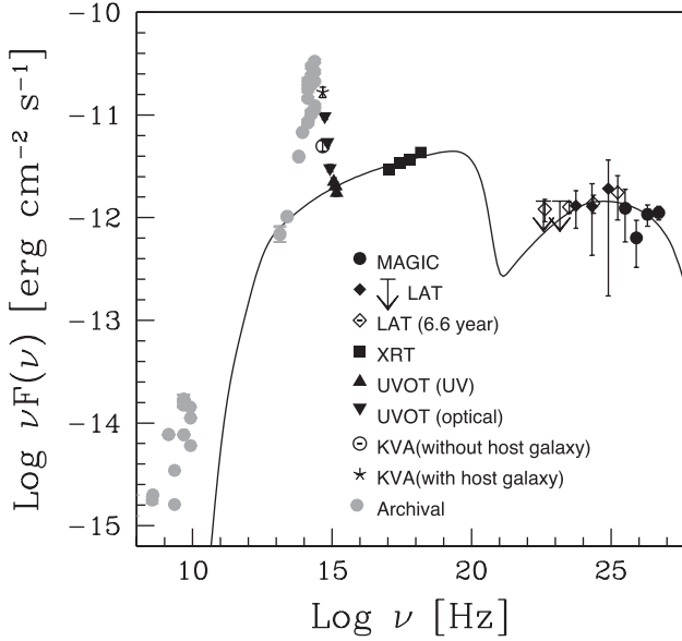
Figure 6. The SED of 1ES 1741+196 from eV to TeV energies. The UV (UVOT UVM1, UVM2, UVW2: filled triangle) fluxes attributed to the nuclear region of blazar are used for the SED fitting – whereas the optical fluxes (KVA: empty circle; UVOT V, B, U: filled inverted triangle) are not. The UVOT UV fluxes are corrected for both the Galactic extinction and the host galaxy, while UVOT optical fluxes are corrected only for the former. The KVA flux with (empty circle) and without (star) subtracting the host galaxy magnitude are also shown. X-ray data (filled square) come from Swift /XRT, averaged over two distinct observations. Contemporaneous (filled diamond) and 6.6 yr-integrated (empty diamond; for comparison) HE \gamma -ray data come from Fermi /LAT. MAGIC data (filled circle) are EBL corrected (Franceschini et al. 2008). We also show the archival data (filled grey circle) for comparison.
