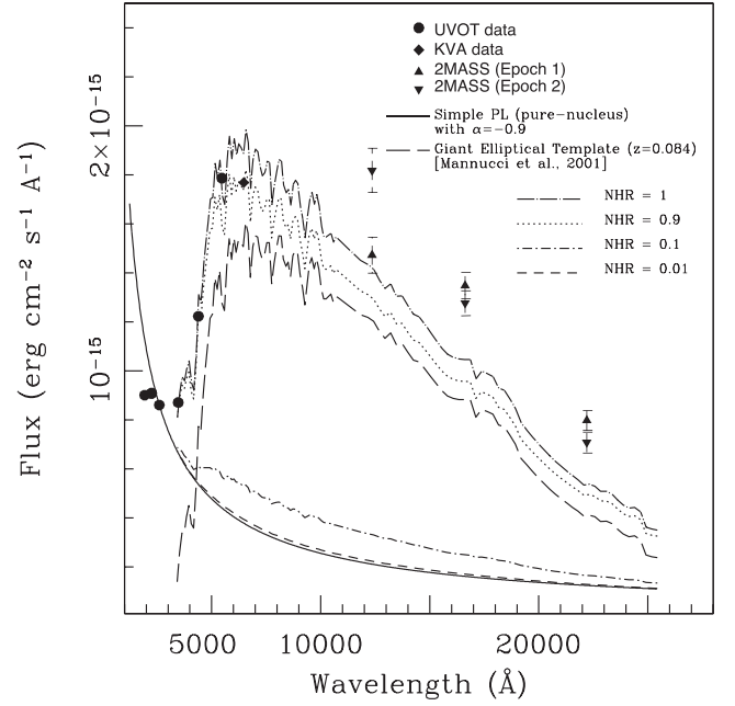
Figure 7. 1ES 1741+196's spectral feature at optical/NIR frequencies, decomposed into blazar and host galaxy components. In the relevant spectral range of interest here, the blazar and the host galaxy are modelled as, respectively, a power law (with a spectral index of 0.9) and a giant-elliptical thermal template (with U - B = 0.50 , B - V = 0.99 , V - R = 0.59 , V - I = 1.22 , V - K = 3.30 ; see Mannucci et al. 2001).
