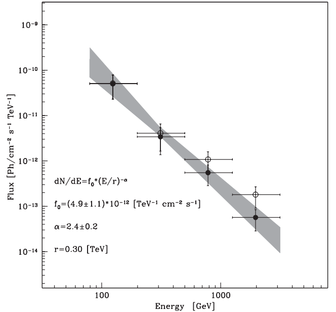
Figure 5. IES 1741+196 differential energy spectrum measured by MAGIC (filled circle), and EBL corrected spectrum using the Franceschini et al. (2008) model (empty circle). The fit function is shown as a grey bow-tie.
