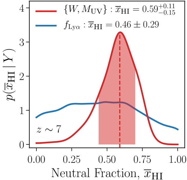
FIG. 11.— Posterior distribution for \bar{x}_{\text{HI}} from the dataset of 68 galaxies at z \sim 7 (including 12 with detected Ly \alpha emission) from Pentericci et al. (2014). In red we plot the posterior distribution obtained from the full sample of \{W, M_{\text{UV}}\} measurements as described in Section 3, and infer a neutral fraction of \bar{x}_{\text{HI}} = 0.59^{+0.11}_{-0.15} (16 – 84%). The dashed line shows the median value, and shaded region shows the (16 th and 84 th ) percentile bounds. For comparison, in blue we plot the posterior for \bar{x}_{\text{HI}} obtained if we used only the fraction of galaxies emitting Ly \alpha with W > 25\text{\AA} , f_{\text{Ly}\alpha} . In this case we infer \bar{x}_{\text{HI}} = 0.46 \pm 0.29 . Using the full distribution of EW provides much more information about the evolving IGM compared to f_{\text{Ly}\alpha} and allows for tighter constraints on the neutral fraction.
