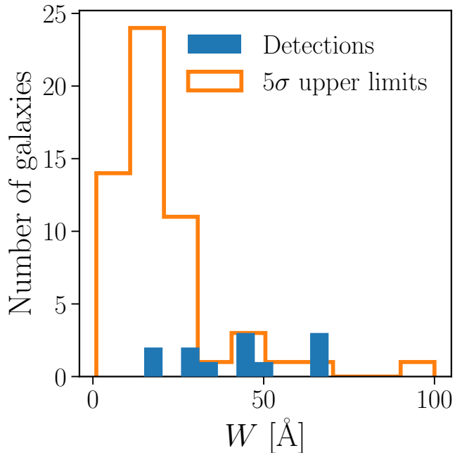
FIG. 10.— EW distribution for the z \sim 7 sample used for the inference. We show both the Ly \alpha EW measurements (filled blue) and 5\sigma upper limits for the non-detections (orange line).
