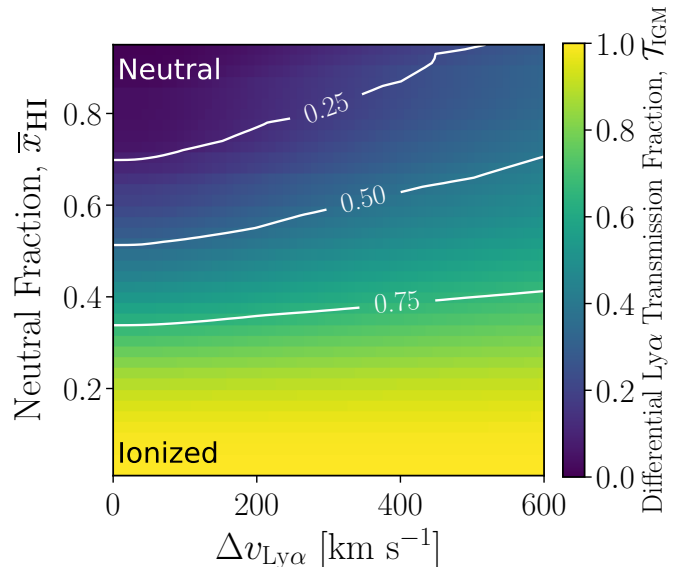
FIG. 5.— Median fraction of Ly \alpha photons transmitted through the IGM, \mathcal{T}_{\text{IGM}} , as a function of \bar{x}_{\text{HI}} and \Delta v computed with Equation 6 from \sim 5000 sightlines to halos with mass 10^{10} M_\odot , assuming \mathcal{T}_{\text{IGM},6} = 1 . Contours show transmission fractions of 25%, 50% and 75%. In a predominantly neutral universe Ly \alpha photons have higher probability of escape through predominately ionized IGM and if emitted at high velocity offsets from their originating galaxies.
