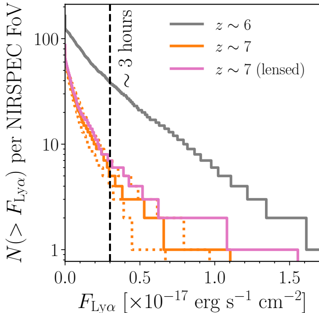
FIG. 13.— Predicted cumulative number counts of LAEs with JWST NIRSpec at z \sim 6 (gray), and z \sim 7 (orange) using our recovered neutral fraction \bar{x}_{\text{HI}} = 0.59^{+0.11}_{-0.15} . Galaxies are drawn from the Mason et al. (2015) UV luminosity function model and populated with equivalent widths via p(W | M_{\text{UV}}, \bar{x}_{\text{HI}}) - the likelihood described in Section 3.1. The number counts obtained within the (16 – 84%) regions on \bar{x}_{\text{HI}} are shown as dotted orange lines. We also show the cumulative number counts for a gravitationally lensed field where we assume a uniform magnification factor of \mu = 2 (pink line), which would reveal more emission lines. We obtain the Ly \alpha fluxes using Equation 14. The dashed black line shows the flux limit for a \sim 3 hour exposure at R = 1000 with JWST NIRSpec F070LP/G140M at 1 - 1.5\mu\text{m} calculated with the JWST ETC ( https://jwst.etc.stsci.edu )
