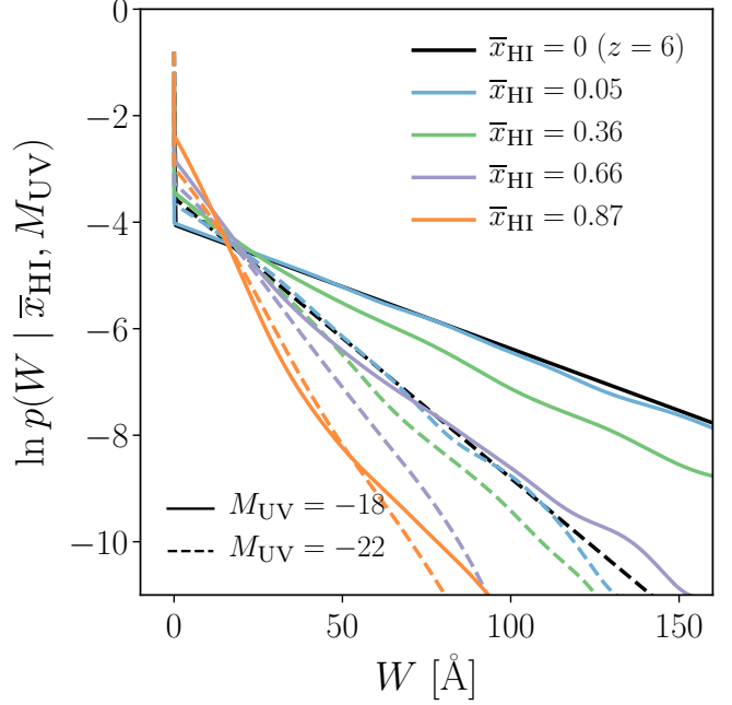
FIG. 7.— Simulated observed distribution of Ly \alpha equivalent widths (the likelihoods for our model) for a range of neutral fractions (colors), for faint (solid line) and bright (dashed line) UV magnitudes. The intrinsic distributions (Equation 4) are shown as black lines. The EW distribution evolves significantly for the UV faint galaxies with increasing \bar{x}_{\text{HI}} , whilst the distribution for UV bright galaxies evolves more slowly.
