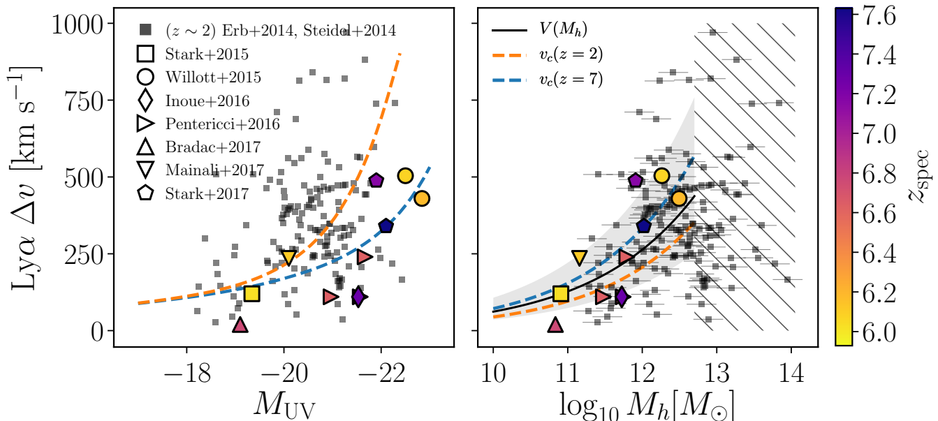
FIG. 2.— Ly \alpha velocity offset as a function of UV absolute magnitude (left), halo mass (right, derived from the Mason et al. (2015) UV magnitude - halo mass relation) for a collection of data from the literature (Erb et al. 2014; Steidel et al. 2014; Willott et al. 2015; Stark et al. 2015, 2017; Inoue et al. 2016; Mainali et al. 2017; Pentericci et al. 2016; Bradač et al. 2017). The gray squares show data from a z \sim 2 sample, whilst the colored points are at z > 6 . We take the z \sim 2 distribution as complete and intrinsic and fit a log-normal distribution to the \Delta v - M_h points as shown in Equation 1. The median \Delta v - M_h fit is shown as a black solid line, and the gray shaded region shows the \sigma_v scatter. We add a 0.2 mag uncertainty to the UV magnitude measurements to account for scatter in the UV magnitude - halo mass relation and use the propagated uncertainties in halo mass in the \Delta v - M_h . The hashed region in the right panel indicates the galaxies with M_{UV} < -21 which are discarded from fitting due to large uncertainties in assigning their halo masses. We plot the circular velocities, v_c of halos at z \sim 2 (dashed orange) and z \sim 7 (dashed blue) for comparison. The \Delta v - M_h relation closely traces the circular velocities, suggesting galaxy mass is a key mediator of Ly \alpha radiative transfer.
