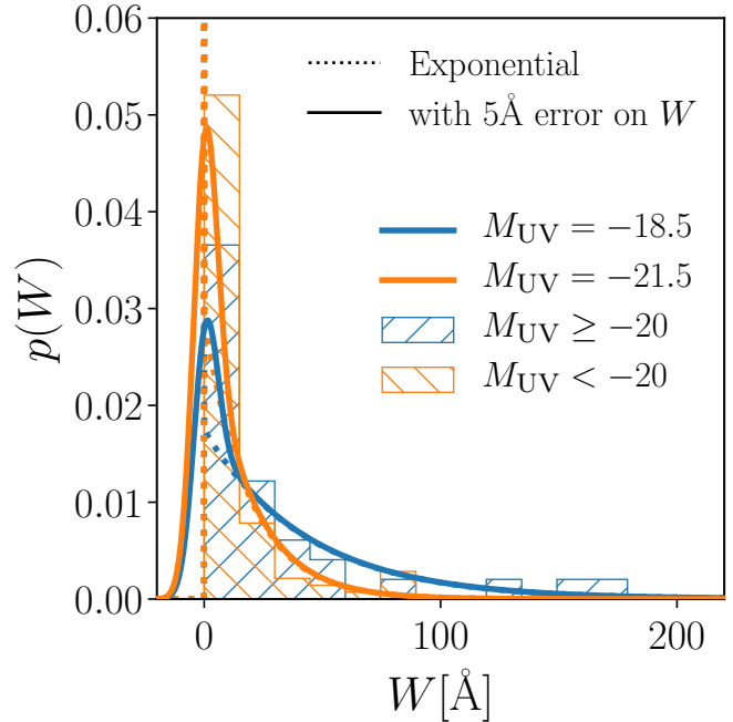
FIG. 3.— z \sim 6 Ly \alpha equivalent width distributions for Lyman Break galaxies given by Equation 4. The dotted lines show the true distribution. For better comparison with the data, we show the PDFs convolved with a 5 \text{Å} typical measurement error on W as solid lines. We plot the PDFs for two values of UV magnitude: M_{\text{UV}} = -18.5, -21.5 (blue, orange). UV faint objects tend to have higher EW and a higher duty cycle of Ly \alpha emission, whereas UV bright galaxies are less likely to emit Ly \alpha and have lower EWs. We also plot the observed EW from De Barros et al. (2017) and Pentericci et al. (2018, in preparation) in UV bright (orange) and UV faint (blue) bins. In these histograms we plot all upper limits at EW = 0 , though note we fully account for upper limits in fitting the EW distribution and the reionization inferences (see Equation 11).
