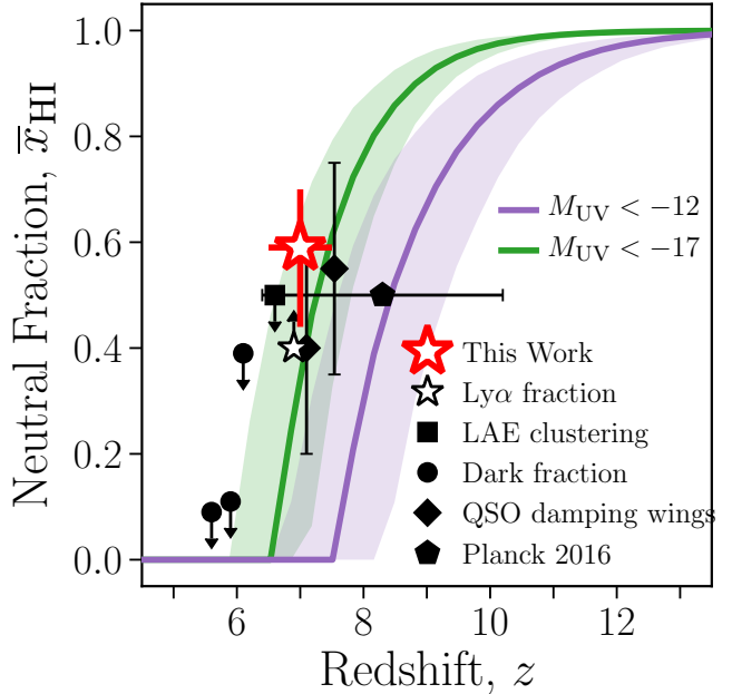
FIG. 12.— The fraction of neutral hydrogen as a function of redshift. Our new constraint is plotted as a red open star. We plot constraints derived from observations of: previous estimates from the fraction of LBGs emitting Ly \alpha (open black star, Mesinger et al. 2015); the clustering of Ly \alpha emitting galaxies (square, Ouchi et al. 2010; Sobacchi & Mesinger 2015); Ly \alpha and Ly \beta forest dark fraction (circle, McGreer et al. 2014); and QSO damping wings (diamond, Greig & Mesinger 2017b; Bañados et al. 2017). We offset the constraints at z \sim 7 (QSO ULASJ1120+0641 damping wing, Greig et al. 2017, Ly \alpha fraction and our new constraint) by \delta z = 0.1 for clarity. We also plot the Planck Collaboration et al. (2016) redshift range of instantaneous reionization (black hatched region). We show as shaded regions the reionization history from integrating the Mason et al. (2015) UV luminosity function to two magnitude limits of M_{\text{UV}} = -17 (green) and M_{\text{UV}} = -12 (purple) and drawing from uniform distributions for the ionizing photon escape fraction 10 – 30% and clumping factor C = 1 - 6 , and log-normal distribution for the ionizing efficiency \xi_{\text{ion}} with mean 25.2 and standard deviation 0.15 dex. There are many uncertainties in obtaining the reionization history from luminosity functions so these should not be taken as real constraints on the neutral fraction, but given that galaxies fainter than M_{\text{UV}} = -17 likely exist (e.g., Kistler et al. 2009; Weisz & Boylan-Kolchin 2017; Livermore et al. 2017; Bouwens et al. 2017b) our result suggests high escape fractions may not be necessary for reionization.
