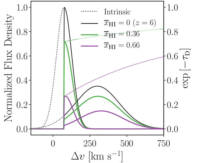
FIG. 1.— The effect of the IGM on simulated line profiles. We show two example intrinsic line profiles (black dotted lines), with peak velocity offsets of 75 and 300 \text{km s}^{-1} , with flux densities normalized to that of the line at 75 \text{km s}^{-1} . This is the line after transmission through the ISM . The solid black shows the lineshape in an ionized universe at z \sim 6 where all flux bluer than the halo’s circular velocity is resonantly absorbed by neutral hydrogen in the local CGM/IGM (i.e. they experience only \tau_{\text{HI}} ). The colored lines show the emission lines after transmission through a reionizing IGM with damping wing optical depths \tau_{\text{D}} , where the median IGM attenuation is also plotted (lighter line, corresponds to right axis). Lines emitted with high velocity offsets are less attenuated by the IGM: for the line with \Delta v = 75 \text{ km s}^{-1} \sim 70\% of the emitted flux is observed for \bar{x}_{\text{HI}} = 0.36 (green), for the line with \Delta v = 300 \text{ km s}^{-1} this fraction rises to \sim 75\% . For \bar{x}_{\text{HI}} = 0.66 (purple) \sim 30\% of the total flux is transmitted from the line with \Delta v = 75 \text{ km s}^{-1} whilst \sim 40\% is emitted for the line at \Delta v = 300 \text{ km s}^{-1} .
