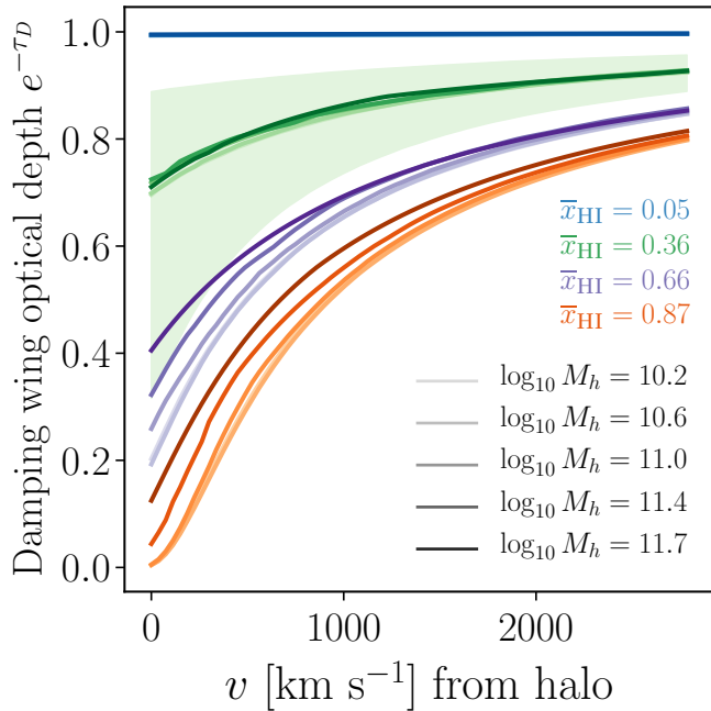
FIG. 4.— Median Ly \alpha IGM damping wing optical depths due to cosmic H I patches during reionization as a function of velocity offset from the center of the source halos. We plot optical depths for 5 different mass halos (indicated by tone of the line - where darkest lines are the highest mass halos) and for 4 volume-averaged neutral fractions \bar{x}_{\text{HI}} (indicated by color). We plot the median optical depth for each halo from the 1000s of simulated sightlines. For \bar{x}_{\text{HI}} = 0.36 we plot the 1\sigma confidence region for the optical depths from all the sightlines to the \log_{10} M_h = 10.2 halos as a shaded area, showing the large variation across sightlines.
