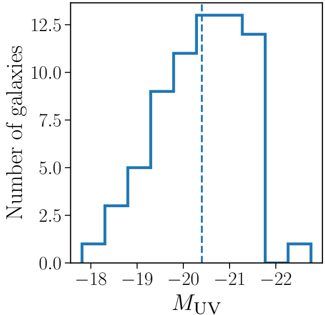
FIG. 9.— UV magnitude distributions for the z \sim 7 sample used for the inference. We plot the median UV magnitude of the sample as a dashed line ( M_{\text{UV}} = -20.4 )
