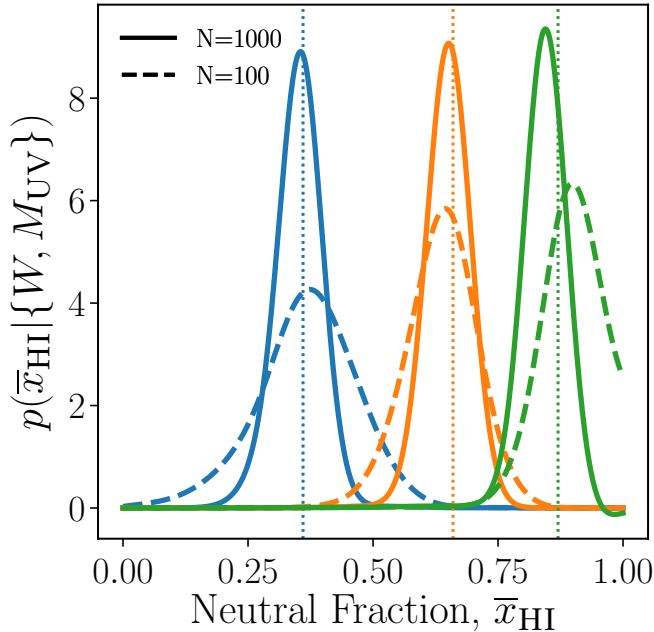
FIG. 8.— Posterior distributions for \bar{x}_{\text{HI}} from simulated samples of Ly \alpha detections from 1000 (solid lines) and 100 (dashed lines) galaxies, for a simulation input value of \bar{x}_{\text{HI}} = [0.36, 0.66, 0.87] (blue, orange, green - the input value is shown by the vertical dotted line). With large samples input neutral fraction is recovered well. With smaller samples, the posterior is wider, but includes the true value within 1\sigma uncertainty.
