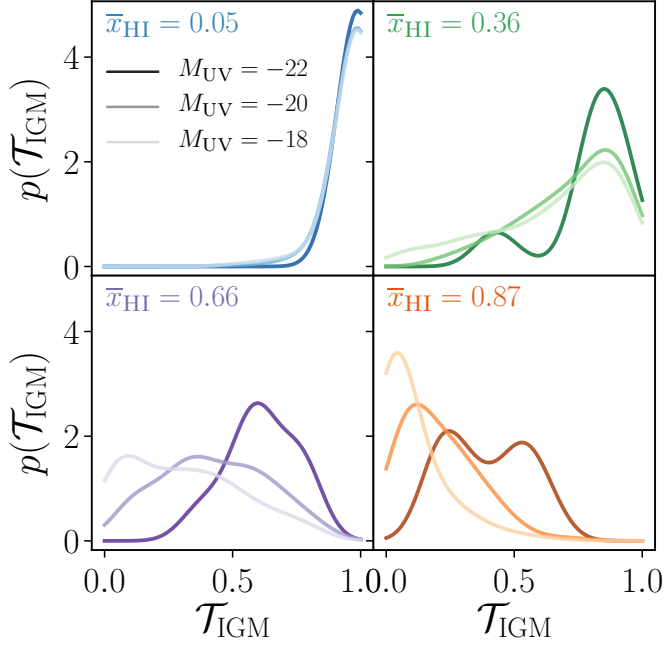
FIG. 6.— Distributions of differential Ly \alpha transmission fractions \mathcal{T}_{\text{IGM}} at z \sim 7 for simulated galaxies of different UV luminosities (UV bright = darkest lines), for a range of IGM neutral fractions \bar{x}_{\text{HI}} . As described in Section 2.2 this is the ratio of Ly \alpha transmission at z \sim 7 to that at z \sim 6 where there is already significant absorption within the ionized IGM (Dijkstra et al. 2007; Zheng et al. 2010; Laursen et al. 2011). The transmission fractions evolve smoothly with the neutral fraction, though the evolution is more gradual for UV bright galaxies.
