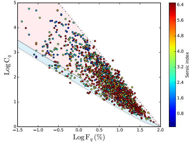
Figure 13. Distributions of MaNGA galaxies on the quiescence ( F_q ) vs. quenching concentration ( C_q ) plane, color-coded according to Sérsic index. Similar to Figure 2, the light blue shaded area denotes the outside-in-like quenching mode whereas the pink shaded region denotes the inside-out-like quenching mode.
