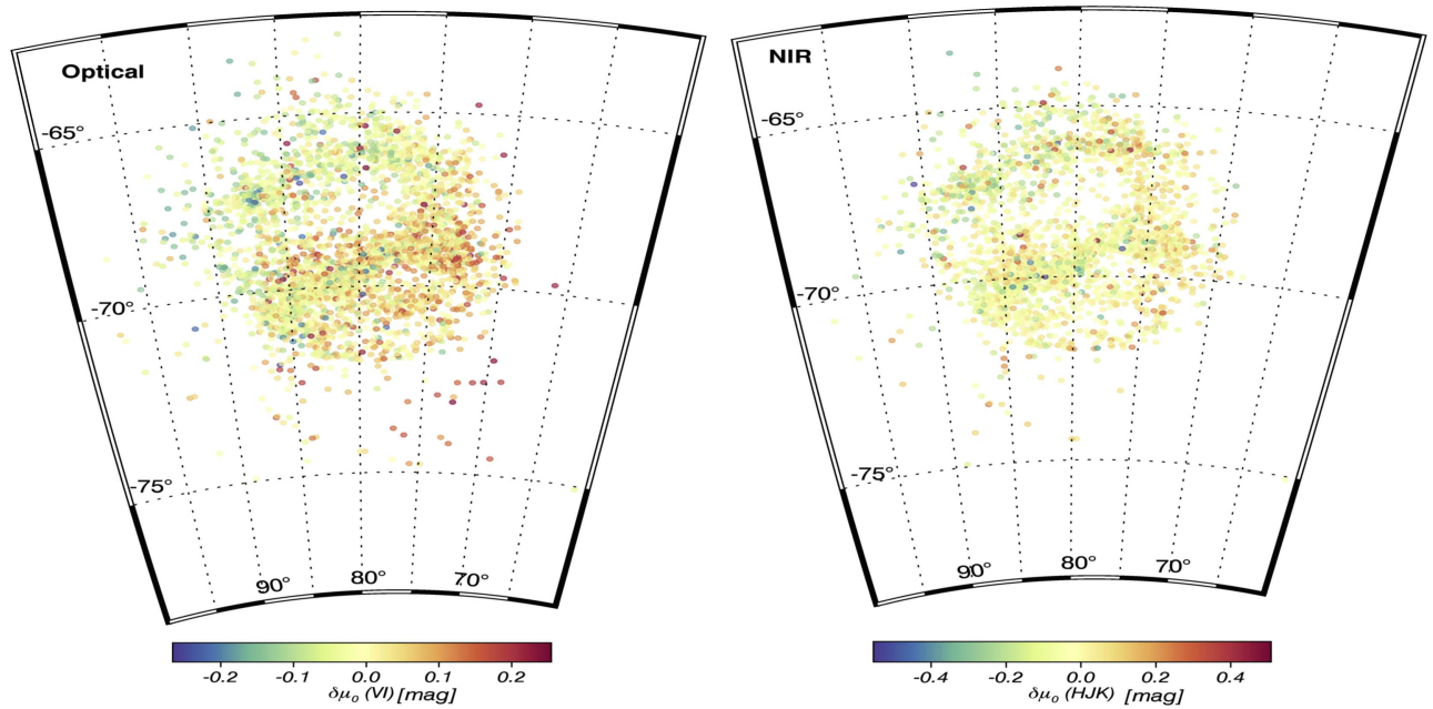
Figure 8. Sky distribution of the Cepheids in Sample A (FU+FO) color coded by their relative distance moduli (mag) obtained by adopting Equations (1) for the optical PW_V relation (left) and the NIR PW_{HJK} relation (right). Both the distributions show similar features, with the eastern part of the LMC closer to us (negative relative distance moduli) with respect to the western region (positive relative distance moduli). The relative distance moduli shown here have been transformed into absolute distances according to Equation (4) and used to derive the viewing angles of the LMC plane.
