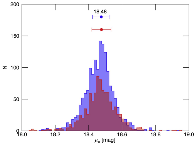
Figure 14. Histogram of the true distance modulus \mu_{0,i} distribution for FU (blue bars) and FO (red bars) Cepheids obtained from Equation (10). The blue dot indicates the median distance from the FU Cepheids’ distribution, while the error bar indicates the 1\sigma dispersion around the median, \sigma = 0.10 mag. The red dot shows the same for FO Cepheids, with \sigma = 0.11 mag. We thus find a median distance modulus to the LMC \mu = 18.48 \pm 0.10 mag for both FU and FO Cepheids. The above value is in excellent agreement with the mean distance modulus by P13, which is accurate to 2.2%.
