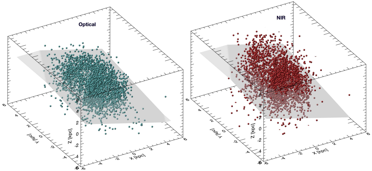
Figure 10. Three-dimensional distribution of the LMC Cepheids in our Sample A. Distances have been determined by adopting the optical PW_{VI} relation (left) and the NIR PW_{HJK} relation (right). The grey shadowed area shows the best-fit plane from which we can derive the LMC viewing angles. A qualitative comparison between the two panels shows that the three-dimensional distribution of the LMC Cepheids as mapped by the optical data is very similar to the one mapped by the NIR ones. However, the larger scatter in z observed in the northern spiral arm for the right panel with respect to the left panel is a consequence of the larger photometric error of the NIR data from the 2MASS subsample with respect to the optical data.
