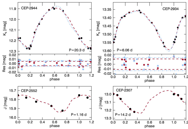
Figure 2. Top—left: comparison between the VMC observations in the K_S band (black solid dots) and two different light-curve fitting functions: a third-order Fourier series (light blue dotted–dashed line) and the template fitting by Inno et al. (2015, red dashed line) for the Cepheid OGLE-LMC-CEP-2944. The residuals between the observed data and the fits are also shown in the lower part of the panel as lightblue dots and as red dots respectively. The dashed lines indicate the rms of the residual, which is larger for the Fourier fitting. Similar results are shown in the right panel for a different Cepheid: OGLE-LMC-CEP-2934, with a shorter pulsation period. Bottom—Template fitting for the five-epochs J -band observations of Cepheids in the VMC sample for a short-period Cepheid (OGLE-LMC-CEP-2552, period \sim 1 day, left panel) and a longer period Cepheid (OGLE-LMC-CEP-2307, period \sim 15 days, left panel). The template fitting correctly recovers the shape of the light curves for FU Cepheids over the whole period range (1–100 days).
