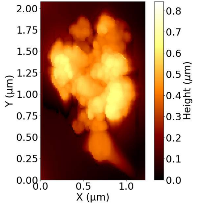
Fig. 9. MIDAS image of an agglomerate particle sticking to the side of a tip that was acquired using a calibration target with sharp spikes (Mannel et al. 2019). The smooth round feature at the bottom is the tip apex, and the straight line to the bottom right corner is a structure supporting the tip. The image has a pixel resolution of about 15 nm and was acquired on 8 December 2015.
