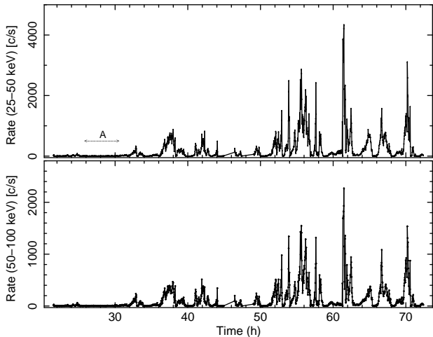
FIG. 1.— Light curve with IBIS/ISGRI count rates in the 25-50 keV and 50-100 keV energy bands, for the data period spanning the revolution 1554. Start time is MJD 57190, UTC 21:30:45:186.
