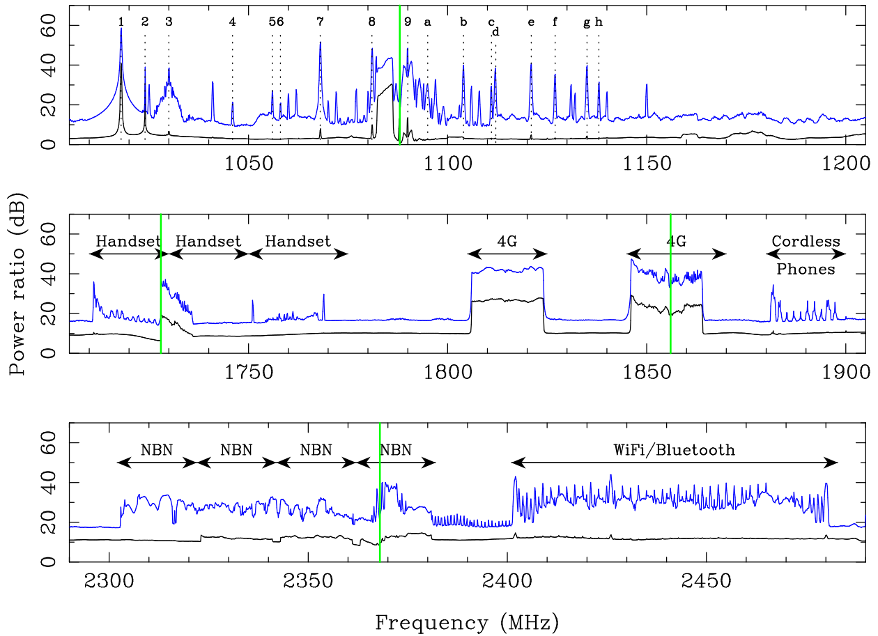
Figure 11. Mean (black line) and peak-hold (blue line) spectra for parts of the band that contain significant impulsive interference. The vertical, green lines indicate sub-band boundaries. Labels in the upper panel indicate DME signals from the following towns and cities: Parkes (1 and 8), Nowra (4 and g), Canberra (5 and h), Sydney (6 and d), Richmond (7), Cowra (a), Williamtown (b), Cooma (c), Wagga Wagga (e) and Albury (f). ADS-B is indicated by 9 and air traffic control ground interrogation by 3. An internal clock system produces signal 2 at 1024 MHz. The broad-signature around 1730 MHz is an alias of strong RFI at the 1860 MHz and the broad signal around 1085 MHz is an alias from a strong mobile-phone band just below 960 MHz. Several of the strong peaks, especially for the peak-hold data in the top panel, have wide sidebands; these originate from the short FFTs used to provide the high time-resolution data.
