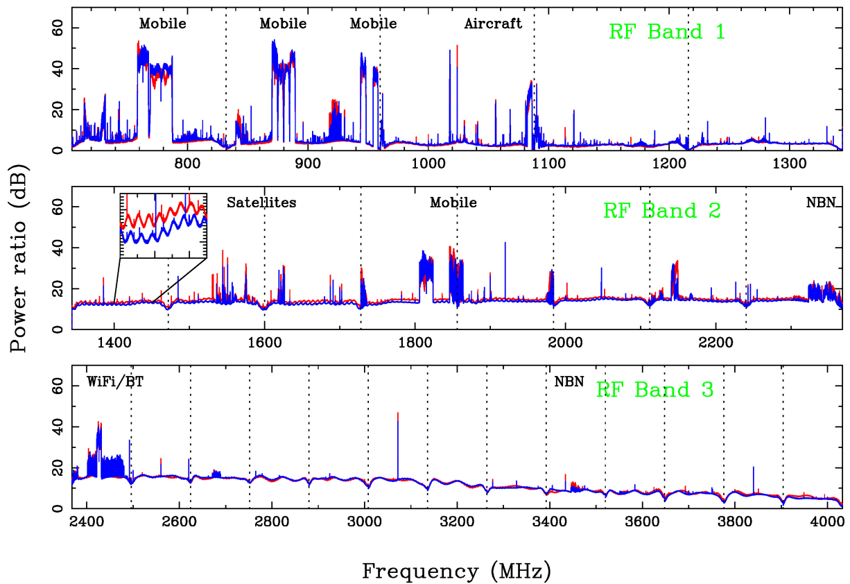
Figure 6. Average spectra across three RF bands obtained on 2019 Feb 24 at 22:48:23 UTC. The red and blue traces represent the A and B polarisations respectively. The vertical, dotted lines indicate the sub-band boundaries and the principal RFI transmissions are labelled. The narrow spikes at 1024, 1920 and 3072 MHz are digital processing artefacts related to the clock signals. NBN stands for the National Broadband Network and BT for Bluetooth. The zoomed-region in RF Band 2 highlights a characteristic ripple that is described in the text. The main text also provides an explanation of the slope across RF Band 3.
