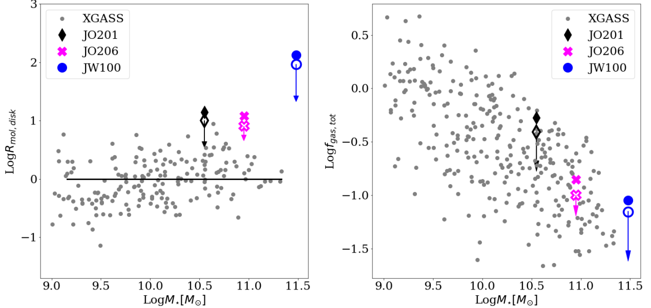
Figure 3. Molecular gas fraction ( R_{mol,disk} = M_{H_2,disk}/M_{HI,disk} ) in the disk (left) and total gas fraction ( f_{gas} = (M_{H_2,tot} + M_{HI,tot})/M_* ) (right) for JO201, JO206 and JW100 compared with the XGASS sample as a function of the stellar mass from Wang et al. 2020; Catinella et al. 2018. The black horizontal line shows the average R_{mol} of the sample.
