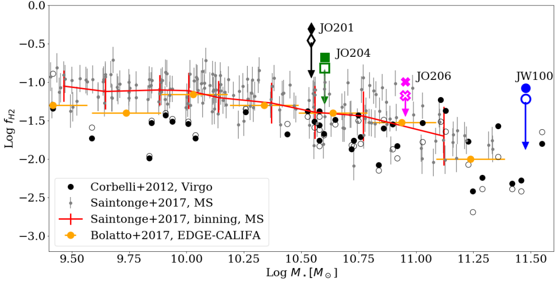
Figure 2. Total molecular gas fraction f_{H_2}(= M_{H_2}/M_*) as a function of the stellar mass. H_2 masses have been derived using a constant \alpha_{CO} (filled symbols) and two different metallicity dependent \alpha_{CO} : the Accurso et al. 2017 (empty symbols) and the Amorin et al. 2016 (arrows). The red line shows the mean scaling relation found in the xCOLDGASS survey by Saintonge et al. (2017) for field galaxies on the main sequence, and grey dots are the single measurements. Orange dots refer to spiral galaxies from the EDGE-CALIFA survey (Bolatto et al. 2017). Black dots are HI deficient galaxies in Virgo from Corbelli et al. 2012: filled symbols and empty symbols represent H_2 masses derived with constant or metallicity dependent \alpha_{CO} .
