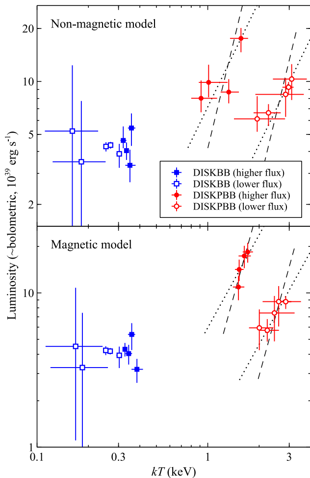
Figure 6. 0.001–100 keV ( i.e. \sim bolometric) luminosity vs temperature for both the DISKBB (blue squares) and DISKPBBS (red circles) components from our multi-epoch spectral analysis with the models assuming the accretor is non-magnetic (top) and magnetic (bottom). No clear relation is seen for the DISKBB component (although this may be related to modelling issues, see Section 4). However, in both cases the results for the DISKPBBS component appear to show distinct tracks at high and low luminosities (observed fluxes above and below F_{0.3-40.0}^{\text{obs}} = 5 \times 10^{-12} \text{ erg cm}^{-2} \text{ s}^{-1} ; full and open symbols, respectively), both of which are broadly consistent with L \propto T^4 (indicated with the dashed lines), and also with L \propto T^2 (dotted lines).
