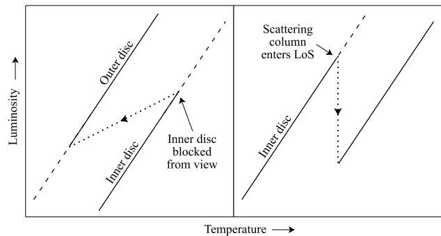
Figure 7. Toy models for the luminosity–temperature plane for the scenarios in which the inner disc is suddenly fully obscured by the outer disc/wind (left panel; discussed in Section 4.2) and in which the emission from the inner disc is scattered by a highly ionised wind which still permits some of the emission to escape (right panel; discussed in Section 4.3).
