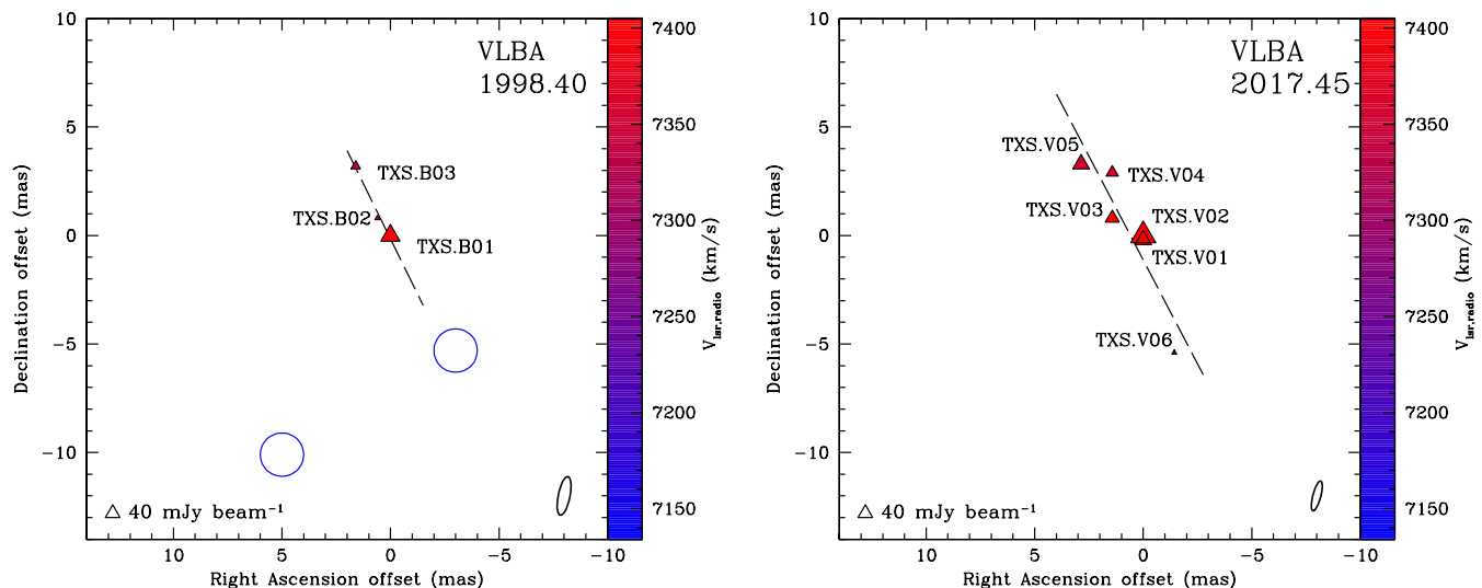
Fig. 2. View of the H 2 O maser features detected towards TXS 2226-184 with the VLBA in epoch 1998.40 ( left panel ) and in epoch 2017.45 ( right panel ). Triangles identify H 2 O maser features whose side length is scaled logarithmically according to their peak flux density (Table 2 and 3). 40 mJy beam -1 symbol is plotted for comparison in both panels. Maser local standard of rest radial velocities are indicated by color (the velocity of the galaxy is V_{\text{lsr,radio}}^{\text{TXS}} = 7270 km s -1 ). The beam size (see Table 1) is shown on the bottom right corner. At the distance of the galaxy (i.e., 107.1 Mpc, derived assuming H_0 = 70 km s -1 Mpc -1 , Kuo et al. 2018) 1 mas corresponds to \sim 0.5 pc. Left panel : in absence of absolute position measurements the relative positions of all maser features are evaluated considering the brightest maser feature (TXS.B01) as reference. The two blue circles indicate the area where Ball et al. (2005) detected the blue-shifted maser features and we did not (detection threshold of 3\sigma ). The dashed line is the best least-squares linear fit of the maser distribution ( \text{PA}_{\text{H}_2\text{O}} = +26^\circ \pm 16^\circ ). Right panel : The reference position is the absolute position of TXS.V02 (see Table 3). The dashed line is the best least-squares linear fit of the maser distribution ( \text{PA}_{\text{H}_2\text{O}} = +28^\circ \pm 12^\circ ).
